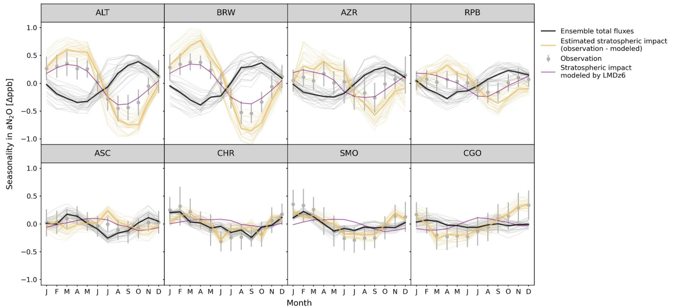
Figure 4. Mismatch (yellow lines) between observed (solid gray circles) and modeled aN_2O seasonality (black lines) at different NOAA/CCGG flask stations (ALT: Alert, BRW: Barrow, AZR: Terceira Island, RPB: Ragged Point, ASC: Ascension Island, CHR: Christmas Island, SMO: Samoa, CGO: Cape Grim) for present day (2001–2020). Thick lines indicate multi-model median and thin lines indicate individual models. Vertical lines on gray circles indicate the standard deviation from temporal variability weighted by measurement uncertainty. The observation-model mismatch (observed—modeled N_2O mixing ratio) provides an estimate of the stratospheric contribution to aN_2O seasonality from N_2O loss and resulting stratosphere-troposphere net fluxes. A modeled stratospheric tracer of N_2O indicating stratospheric contribution for the same period using the chemistry-transport model, LMDz6 (see Ruiz and Prather (2022) for methods), is shown in purple lines for comparison.
