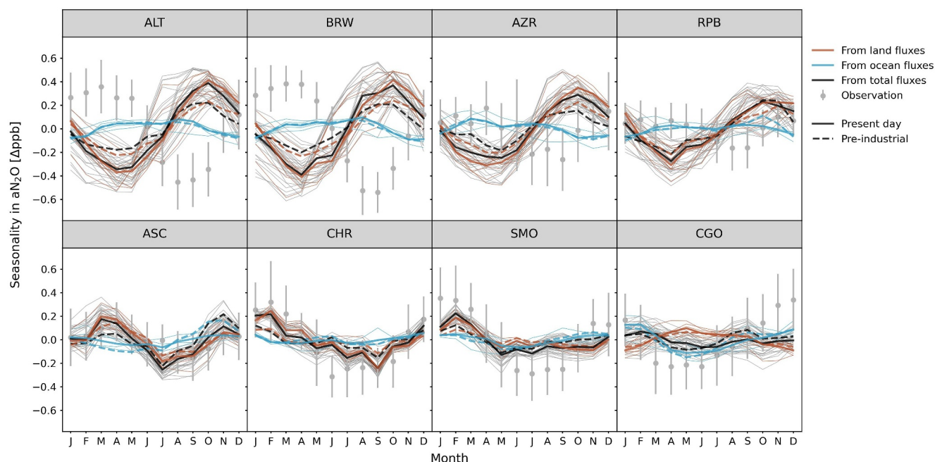
Figure 5. Long-term average seasonality of observed \text{aN}_2\text{O} (solid gray circles) and modeled \text{aN}_2\text{O} (lines) at different NOAA/CCGG flask stations (ALT: Alert, BRW: Barrow, AZR: Terceira Island, RPB: Ragged Point, ASC: Ascension Island, CHR: Christmas Island, SMO: Samoa, CGO: Cape Grim). Modeled \text{aN}_2\text{O} seasonality is attributed to the \text{N}_2\text{O} emissions from the land (solid red lines) and the ocean (solid blue lines), and total emissions (solid black lines) for present day (2001–2020). Only the multi-model median of \text{aN}_2\text{O} seasonality for the pre-industrial period (1861–1880) is given (dashed lines). Thick lines indicate multi-model median and thin lines indicate individual models. Vertical lines on gray circles indicate observed temporal variability weighted with measurement uncertainty.
