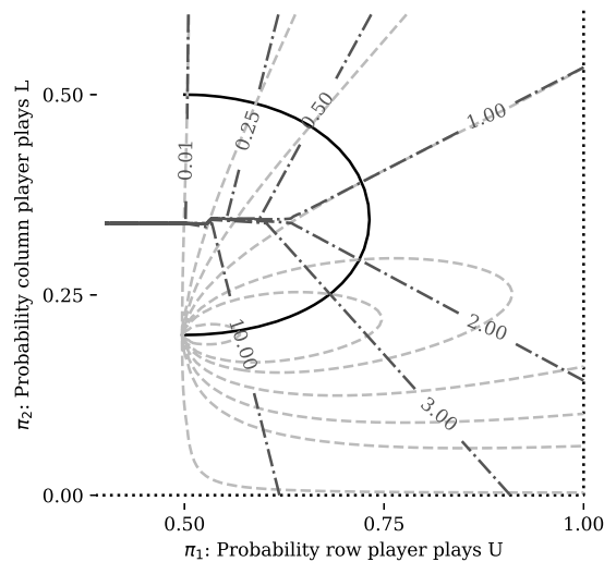
Fig. 6. Level sets of \hat{\lambda}^{EC} and \hat{\lambda}^{EP} for various values of \lambda for the Ochs game in Table 3a. The solid line is the locus of LQRE profiles for the base game. The darker dot-dashed lines correspond to level sets of \hat{\lambda}^{EC} , and lighter dashed lines to level sets of \hat{\lambda}^{EP} . For a given common \lambda , the level sets of EC and EP intersect at the point where they cross the locus of profiles.
