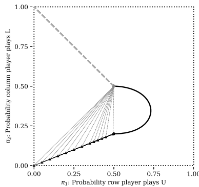
(b) Best response (D, R) .
