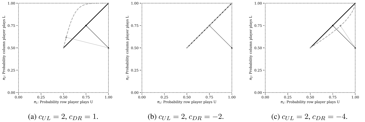
Fig. 7. Examples of the three cases for the family of games in Table 5. The empirical strategy frequencies illustrated are (1, \frac{1}{2}) for all three examples, all of which are mapped to (\frac{3}{4}, \frac{3}{4}) by the equilibrium correspondence approach.
