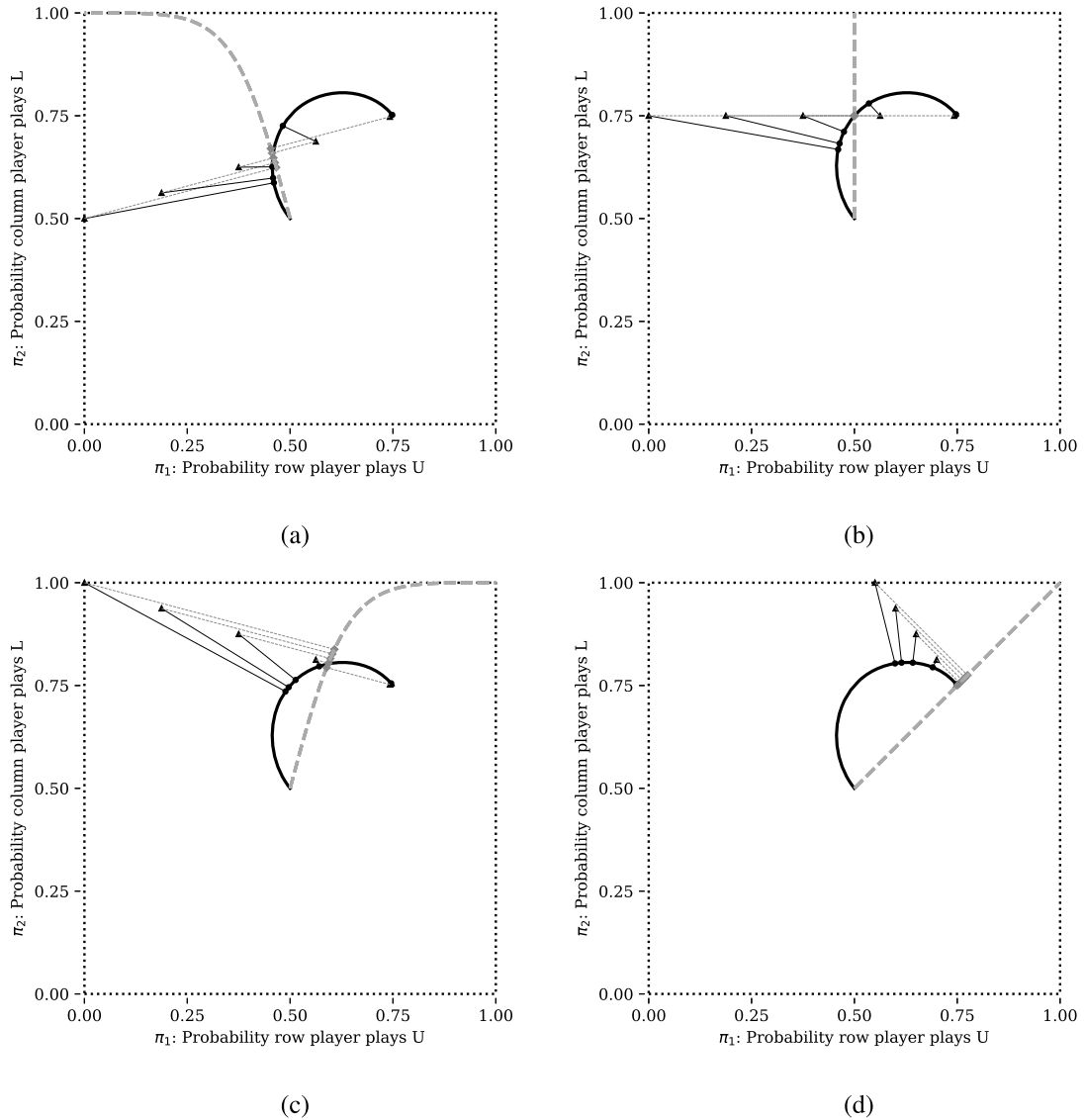
Fig. 5. Four examples of comparative statics of \hat{\pi}^{EC} and \hat{\pi}^{EP} for the generalized matching pennies game in Table 4.
