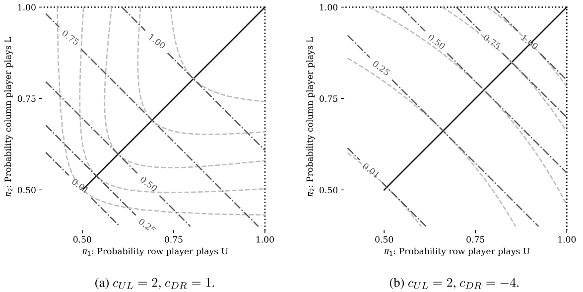
Fig. 8. Level sets of \hat{\lambda}^{EC} and \hat{\lambda}^{EP} for games from Fig. 7 with symmetric LQRE profiles. The solid line is the locus of LQRE profiles for the base game. The darker dot-dashed lines correspond to level sets of \hat{\lambda}^{EC} , and lighter dashed lines to level sets of \hat{\lambda}^{EP} .
