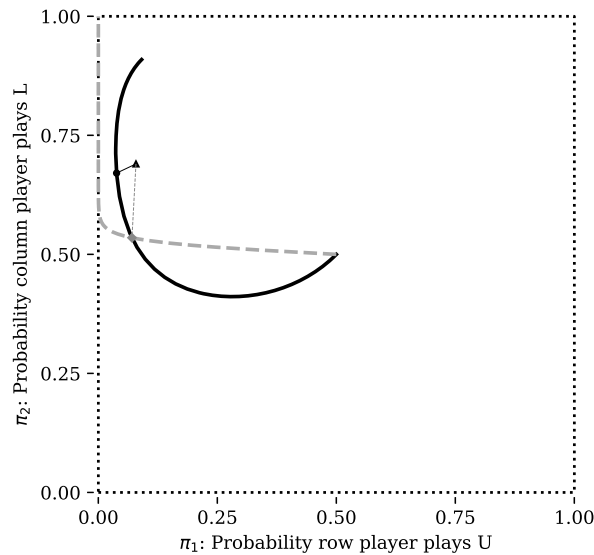
Fig. 1. Data and estimation results for Game 1 from Selten and Chmura (2008). The empirical strategy probabilities are represented by the triangle. The locus of LQRE profiles of the base game is represented by the darker solid curve, and that of the auxiliary game by the lighter dashed curve. The dots indicate the corresponding maximum likelihood estimates for the two approaches.
