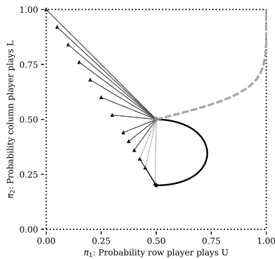
(a) Best response (D, L) .
