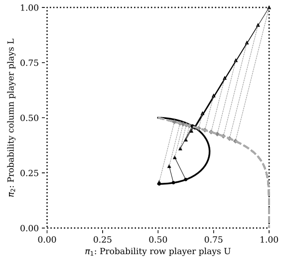
(b) Observed data \frac{u_U(p) - u_D(p)}{u_L(p) - u_R(p)} = -4 .
