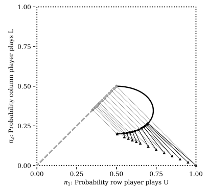
(c) Best response (U, R) .
