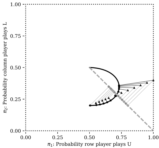
(a) Observed data \frac{u_U(p) - u_D(p)}{u_L(p) - u_R(p)} = -1 .
