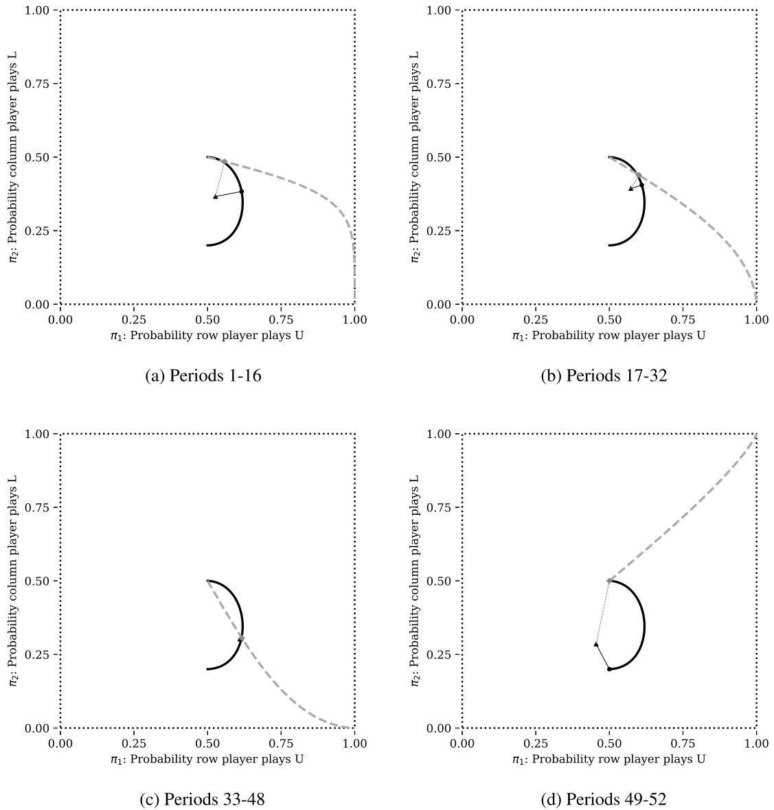
Fig. 2. Graphical comparison of LQRE analysis of Table 3 via the equilibrium correspondence and empirical payoff approaches. The solid curve is the locus of LQRE profiles of the base game. The triangle indicates the location of the empirical frequencies of play. Each dashed curve represents the locus of LQRE profiles of the auxiliary game arising from the empirical data. Dotted lines connect the empirical data to the fitted profiles on the loci of the respective approaches.
