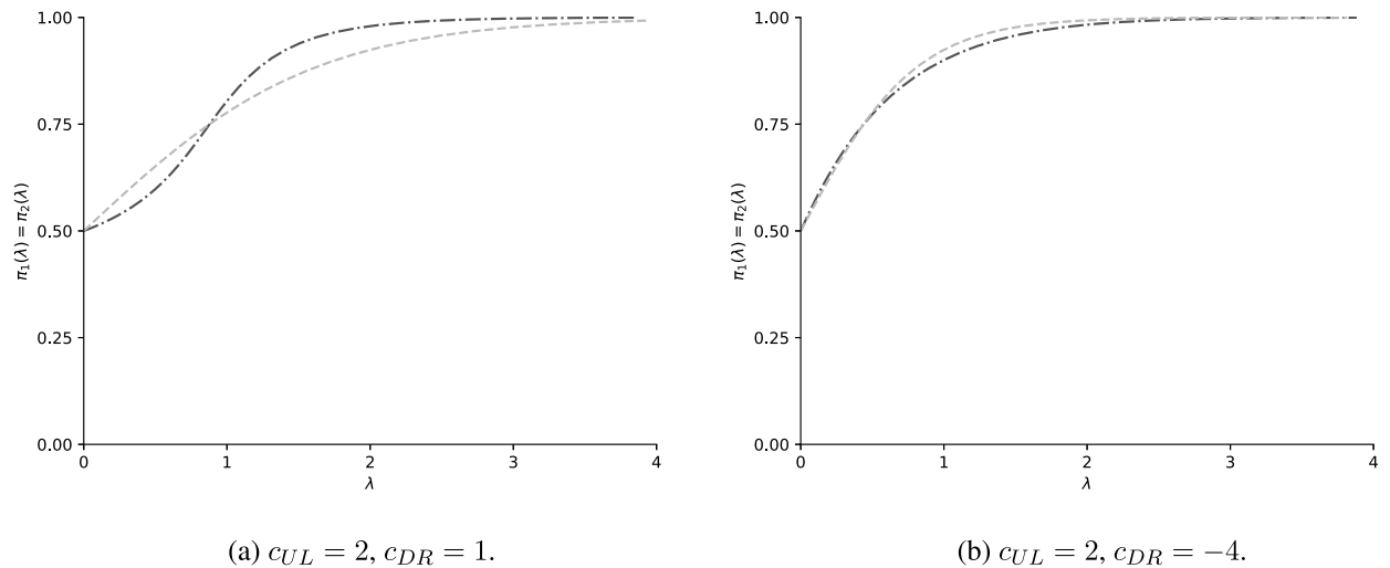
Fig. 9. Correspondence plots of \pi_1^{EC}(\lambda) = \pi_2^{EC}(\lambda) and \pi_1^{EP}(\lambda) = \pi_2^{EP}(\lambda) for games from Fig. 7 with symmetric LQRE profiles, given observed strategy frequencies p_1 = p_2 = \frac{3}{4} . The darker dot-dashed lines correspond to the correspondence \pi^{EC} , and lighter dashed lines to \pi^{EP} .
