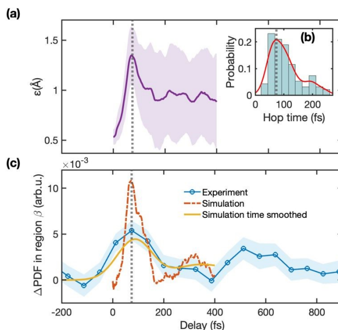
Figure 6: Ring stretching motion dynamics reflected in the experiment and simulated \Delta PDF s. Panel (a) shows the amount of ring stretching averaged over the simulated trajectories as a function of time delay ( \varepsilon_{avg}(t) ) along with the standard deviation from the mean. The inset (b) shows the probability distribution of hop times from S_1 to S_0 (excited-state to ground-state) for all trajectories. Panel (c) shows the sum of \Delta PDF intensity in the region \beta ( 2.6 < r(\text{\AA}) < 3 ) for the experiment (blue) along with the one-standard-deviation error (shaded region), the corresponding signal from the simulation without (red) and with (yellow) 150 fs gaussian time smoothing applied. The vertical grey dotted line in Panels (a), (b), and (c) marks the most likely time (74 fs) for the wavepacket to reach the CI seam.
