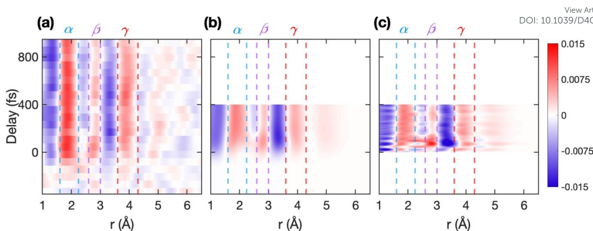
Figure 3: Experiment and simulated \Delta PDFs. The false color plots show the difference diffraction signal ( \Delta PDF ( r , t )) in real space as the function of pump-probe delay for (a) experiment, (b) (scaled) simulation convolved in time with a Gaussian of 150 fs full width at half maximum (FWHM), and (c) (scaled) simulation without any convolution in time. The regions \alpha ( 1.6 < r(\text{\AA}) < 2.25 ), \beta ( 2.6 < r(\text{\AA}) < 3 ), and \gamma ( 3.6 < r(\text{\AA}) < 4.3 ) are marked in all three panels with blue, purple, and red broken lines, respectively. The \Delta PDF in region \beta ( 2.6 < r(\text{\AA}) < 3 ) has a modulation in intensity with the delay.
