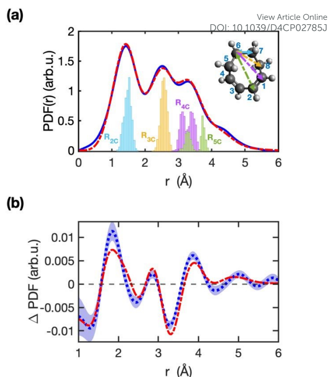
Figure 2: Comparison of experimental and simulated diffraction signals in real space. Panel (a) shows the experimental (blue-solid line) and simulated (red dashed line) stationary ground-state PDF( r ) of COD. The blue, yellow, purple, and green histograms in panel (a) depict the distribution of carbon-carbon distances of the geometries in the TSH simulations at time-zero, for the ground-state Wigner ensemble. The inset illustrates the averaged stationary-ground state molecular structure (at T = 0 fs) with different carbon-carbon distances marked in color code for one of the carbon atoms in the molecule ( R_{2C} , R_{3C} , R_{4C} , and R_{5C} distances are marked in blue, yellow, purple, and green arrows, respectively). Panel (b) shows the experimental (dotted blue line) and simulated (dashed red line) \Delta PDF averaged over delays between 250 fs to 400 fs. The shaded blue area in panel (b) represents the statistical one-standard deviation error of the experiment signals calculated from a bootstrap analysis.
