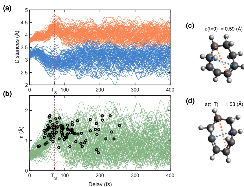
Figure 5: Ring distortion motion. Panel (a) shows the changes in largest ( [R_{5C}]_{\max} ) and shortest ( [R_{5C}]_{\min} ) R_{5C} distances of all the 95 trajectories used in calculation of simulated signal, in orange and blue, respectively, as a function of delay for the first 400 fs. Panel (b) shows the evolution of the ring distortion motion parameter ( \varepsilon(t) ), which is equal to the difference of [R_{5C}]_{\max} , and [R_{5C}]_{\min}(t) . The \varepsilon(t) values of all the 95 trajectories used for calculating simulated signal are shown in this plot. The black circles represent the S_1 \rightarrow S_0 hop times of the trajectories. The vertical dotted line (in maroon) in panels (a) and (b) corresponds to the time T_S ( t = 70 fs) at which maximum ring stretching motion is observed over all the 95 trajectories. Panels (c) and (d) show representative structures from a trajectory simulation at t = 0 and T_S ( t = 70 fs) respectively, as an example to show the amount of ring stretch present. The largest and shortest R_{5C} distances are marked with orange and blue lines, respectively, and
