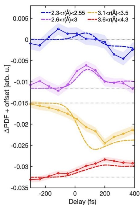
Figure 4: Comparison between experiment and simulated \Delta PDF signals at different regions. The lineouts in blue, purple, yellow, and red colors represent the summed \Delta PDF signal in regions of 2.3 < r(\text{\AA}) < 2.55 , 2.6 < r(\text{\AA}) < 3 , 3.1 < r(\text{\AA}) < 3.5 , and 3.6 < r(\text{\AA}) < 4.3 , respectively. The experiment signals are depicted by solid lines with circle markers, and the simulated signals are illustrated with broken lines. The shaded area in all panels represents the statistical ( 1-\sigma ) error of the experiment signals for the corresponding region, calculated from a bootstrap analysis. An offset in the y-axis is added to the lineouts to displace them vertically for visualization. Each feature is plotted relative to the offset added. The offset is marked in grey dotted lines.
