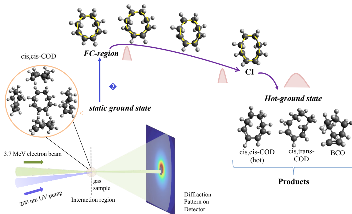
Figure 1: Schematic illustrating the UED experimental set-up and the photoinduced structural dynamics of cc-COD. The cc-COD molecules in the gas phase are introduced in the interaction region via a flow cell. The inset shows the randomly oriented cc-COD molecules. A 200 nm UV pump pulse is used to excite the cc-COD molecules from the static ground state, and 3.7 MeV electron pulses with a variable time delay are used to probe the molecules. The scattered diffraction patterns are recorded on the detector. The structures of the molecule in the static ground state/ FC-region ( t = 0 fs), in the excited-state at t = 20 fs, t = 40 fs, and at a conical intersection seam ( t = 74 fs) are shown. The qualitative depiction of ring distortion motion (highlighted in yellow) in the molecule, as it approaches the CI seam, is shown along with the width of the nuclear wavepacket (in light red), which remains compact until the CI seam is reached and spreads out rapidly after passing through the CI seam and into the ground state where multiple products are formed. Representative structures of the photoproducts predicted from our TSH theoretical simulations at a pump-probe delay of 350 fs are shown. The products are cc-COD, ct-COD, and BCO, and their calculated yields (at t \sim 400 fs) from TSH simulations are 63 %, 32%, and 5%, respectively.
