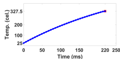
Fig. 8: The temperature characteristic of the welding load (the welding lead) during the pre-welding period at a firing angle of 40% (108 degrees).
