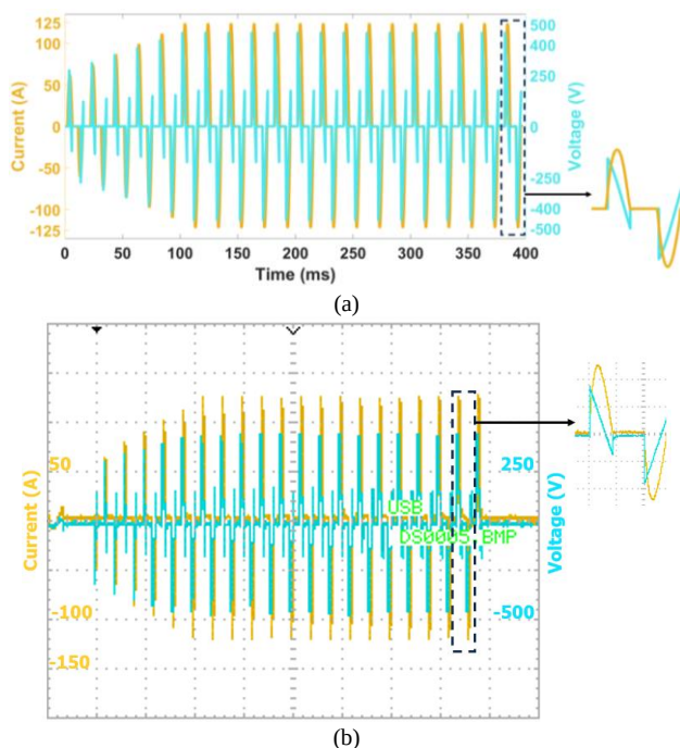
Fig. 7: Input voltage (blue) and input current (yellow) of the transformer at a frequency of 50 Hz and firing angle of 30%: (a) simulation; (b) Experimental (each division on the oscilloscope corresponds to 250 V / 50 A).
