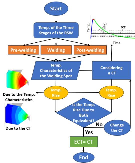
Fig. 13: The process of obtaining ECT (CT: a constant temperature).
