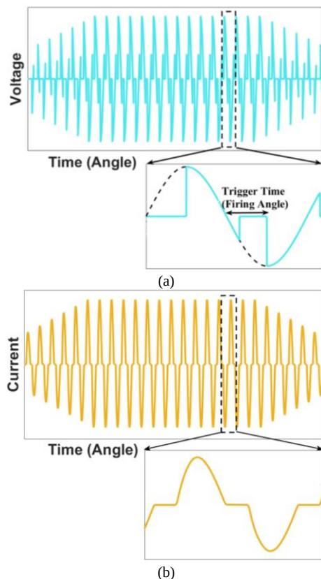
Fig. 2: General representation of voltage and current in a WT: (a) applied voltage; (b) supply current.
