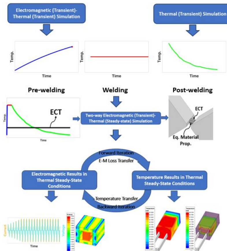
Fig. 5: The proposed FEM-based multi-physics approach for determining the steady-state characteristics of the RSW transformer.
