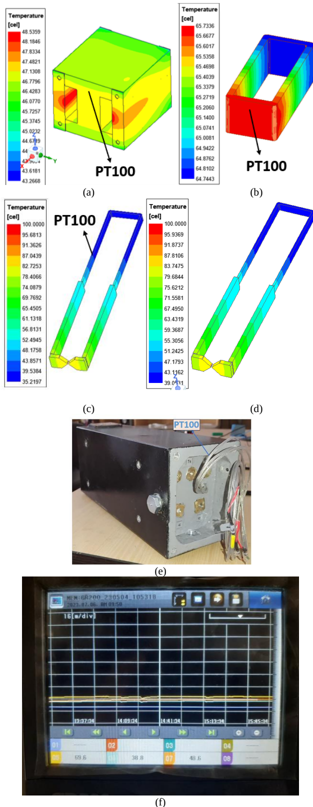
Fig. 15: The steady-state temperatures of the fabricated transformer components for an input of 20 voltage cycles with a firing angle of 40% and a rest period of 4.8 s: (a) core; (b) primary winding; (c) secondary winding (ingot) for an ideal cooling water pipe without deposits; (d) secondary winding (ingot) for the cooling water pipe with a 50% reduction in the effective cross-sectional area due to sedimentation; (e) the fabricated RSW transformer, along with the incorporated PT100 temperature sensors; (f) the steady-state temperatures recorded by the PT100 sensors. Channels: primary winding (yellow), secondary winding (blue), and core (orange).
