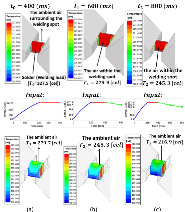
Fig. 11: The first three steps of determining the temperature of the air at the welding spot (between the electrodes) during the post-welding stage. Determination of: (a) T_1 ; (b) T_2 ; (c) T_3 (also see Table I).
