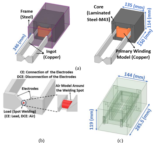
Fig. 4: The RSW transformer model: (a) transformer components; (b) welding spot load; (c) resin mold of the transformer.
