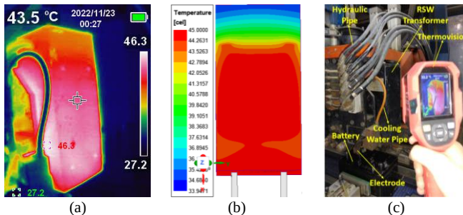
Fig. 14: Steady-state temperature of the RSW transformer frame for an input of 20 voltage cycles with a firing angle of 40% and a rest period of 4.8s: (a) experimental; (b) simulation; (c) the components in the welding line.
