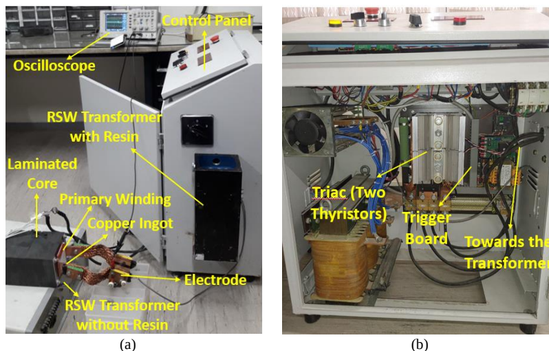
Fig. 6: Experimental test setup. (a) The test setup for RSW transformer. (b) Control panel components.
