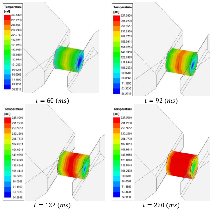
Fig. 9: The characteristic temperature contour of the welding lead during the pre-welding period at a firing angle of 40%.
