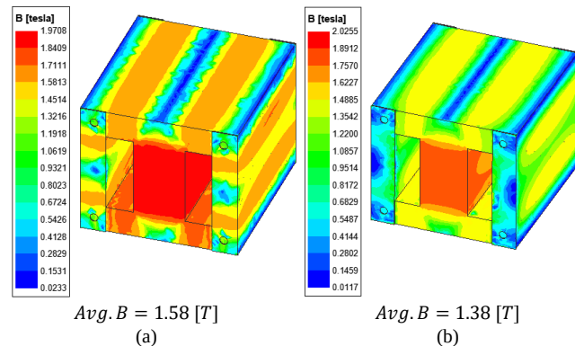
Fig. 17: The maximum magnetic flux density of the transformer core: (a) electro-magnetic analysis; (b) electro-magnetic-thermal analysis.
