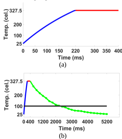
Fig. 10: The characteristic temperature of the welding spot and its ECT. (a) The characteristic temperature of the welding lead during the pre-welding (blue) and welding (red) period for the 20 welding voltage cycles at the firing angle of 40%; (b) the temperature characteristic of the welding spot (between the electrodes) during a complete welding cycle of a battery strap for 20 cycles at a 40% firing angle voltage: pre-welding (blue), welding (red), post-welding (green), and ECT (black).
