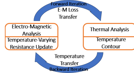
Fig. 3: Two-way electromagnetic-thermal analysis process.
