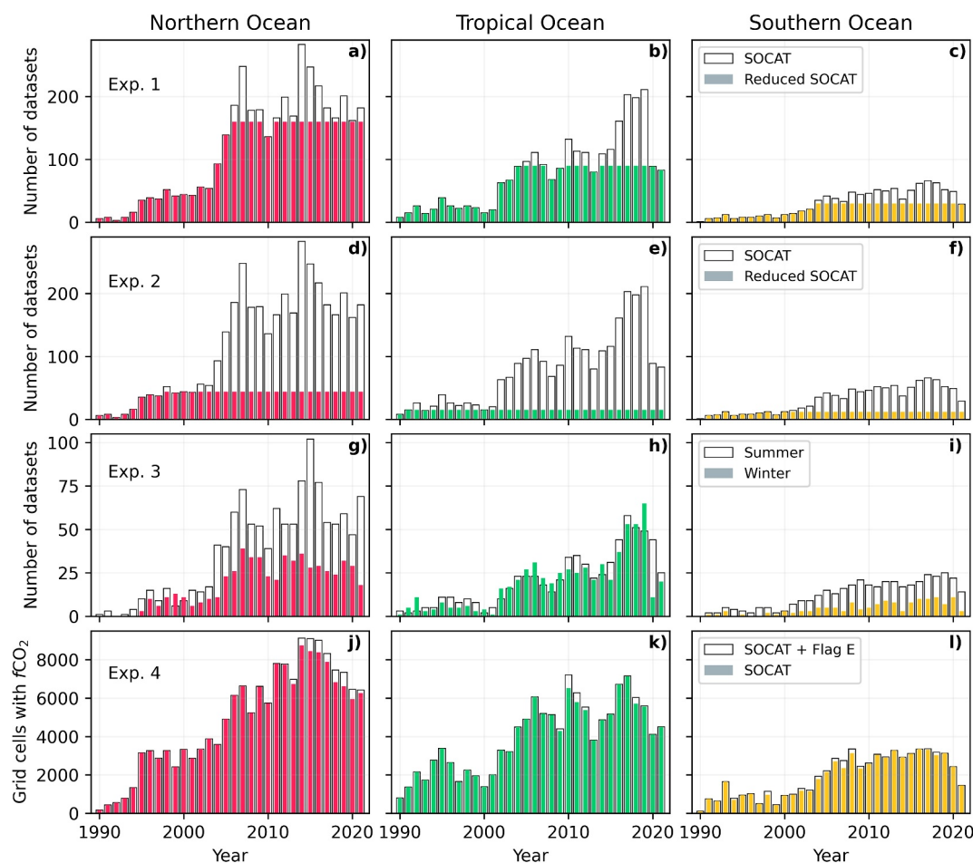
Figure 1. The number of data sets or grid cells with f\text{CO}_2 in SOCATv2023 for each year from 1990 to 2021. The left, middle, and right panels represent the Northern, Tropical, and Southern Oceans, respectively. (a–c) White bars represent the number of data sets in Surface Ocean \text{CO}_2 Atlas (SOCAT), and shaded bars denote the number of remaining data sets after the removal of some data sets to match a similar number in 2021 (see Section 2, experiment 1). (d–f) White bars represent the number of data sets in SOCAT while shaded bars correspond to the number of the remaining data sets after removal of data sets more than the number of those in the year 2000 (see Section 2, experiment 2). (g–i) White and shaded bars indicate the number of data sets in summer and winter, respectively (see Section 2, experiment 3). (j–l) Solid bars represent the number of monthly grid cells with f\text{CO}_2 with an estimated accuracy better than 5 \mu\text{atm} in SOCAT, while white bars indicate the number of grid cells upon addition of lower accuracy data sets with a flag of E (see Section 2, experiment 4). The white bars in all subplots start at the bottom (i.e., zero).
