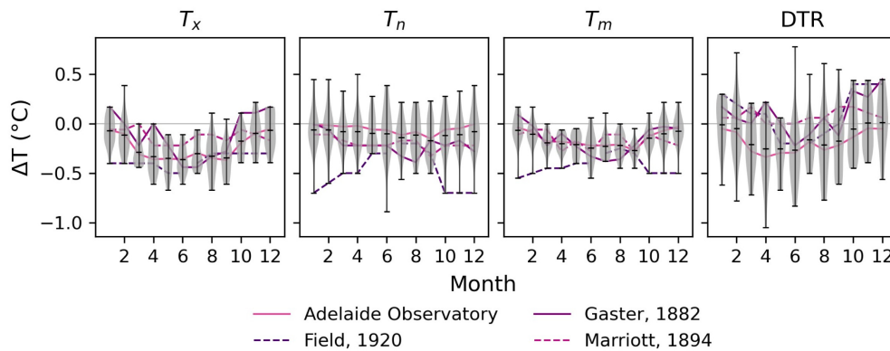
FIGURE 5 As Figure 3, but for differences between Stevenson screens and intermediate exposures.
