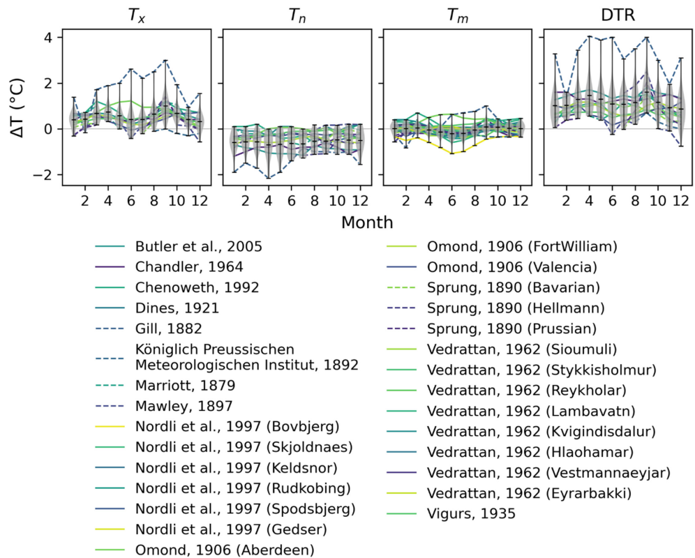
FIGURE 4 As Figure 3, but for differences between Stevenson screens and wall-mounted exposures.
