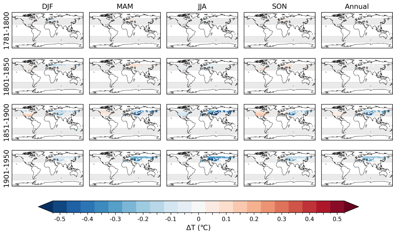
FIGURE 13 Difference between CRUTEM5_ext and CRUTEM5_eba seasonal and annual means over time ( \Delta T = \text{CRUTEM5\_eba} - \text{CRUTEM5\_ext} ).
