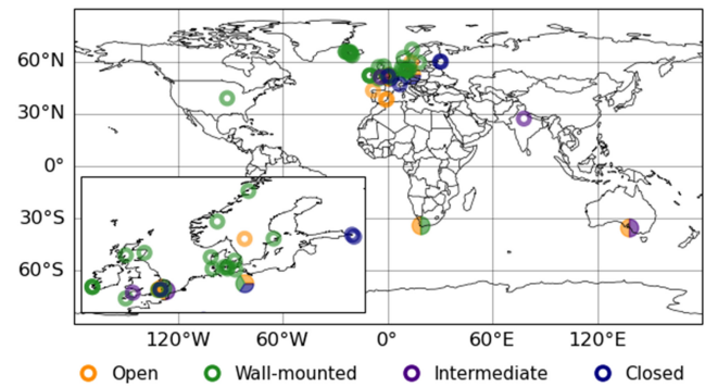
FIGURE 2 Locations of the parallel measurement series collated and analysed.
