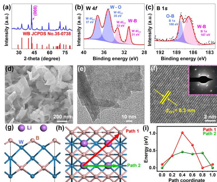
Fig. 3. (a) XRD pattern of WB. XPS spectra of (b) W 4f and (c) B 1s of WB. (d) SEM image, (e) HRTEM image, and (f) a high-magnification HRTEM image with an inset of SAED pattern of WB. (g) Simulated \text{Li}^+ ion diffusion on the WB. Schematic showing (h) the Path1 and Path2 diffusion path and (i) corresponding activation energy profile.
