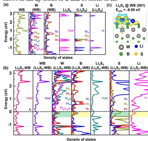
Fig. 2. The DOS (a) of pure WB and \text{Li}_2\text{S}_4 . The DOS (b) and binding energy value (c) of \text{Li}_2\text{S}_4 adsorbed on the WB (001) surfaces.
