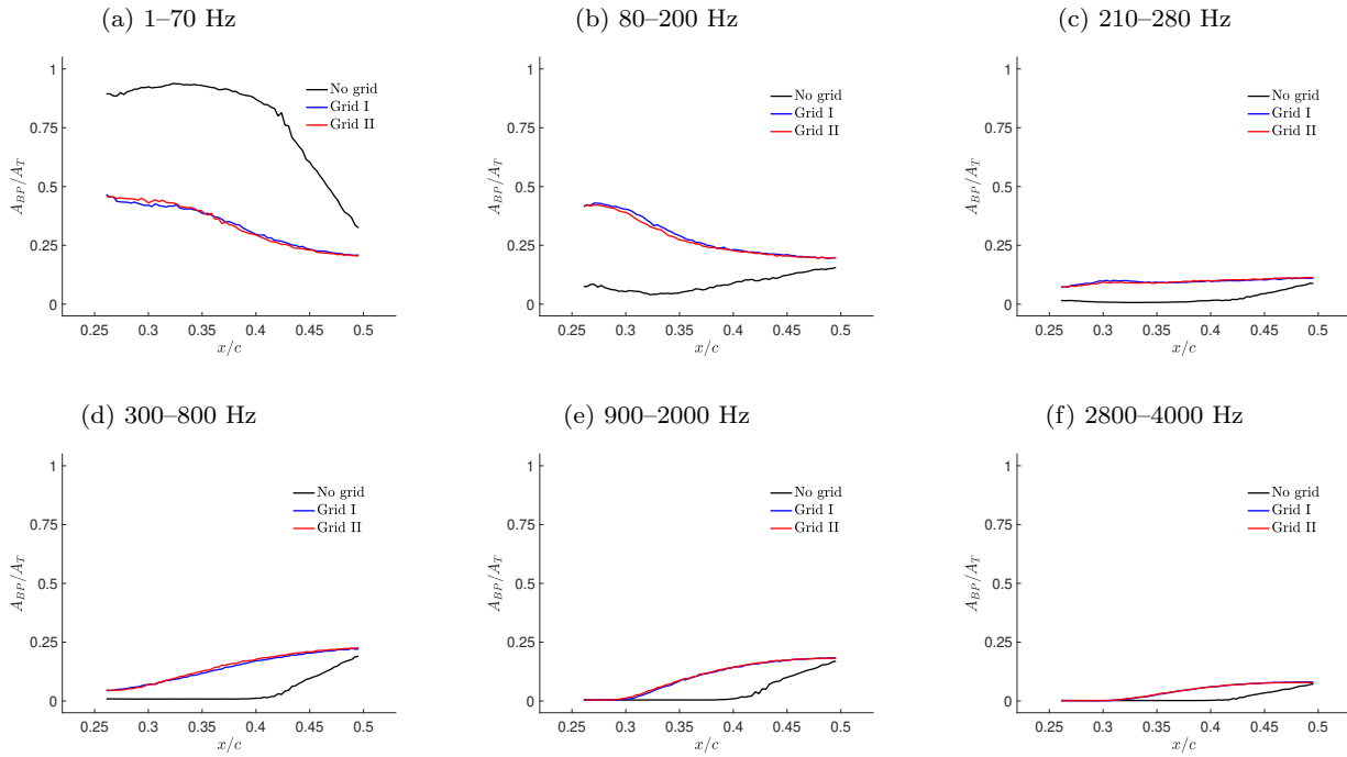
Fig. 12 Bandpass-filtered disturbance amplitude for waves within different frequency ranges. Bandpass-filtered amplitudes are normalised with the overall disturbance amplitude, A_T .
