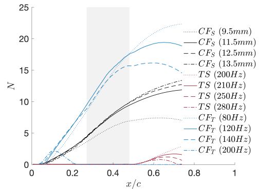
Fig. 3 N -factor curves obtained from linear stability analysis with the measured experimental pressure distribution in figure 2. The grey shaded area indicates the location of the hot-wire measurements. The data are taken from van Bokhorst (2018).
