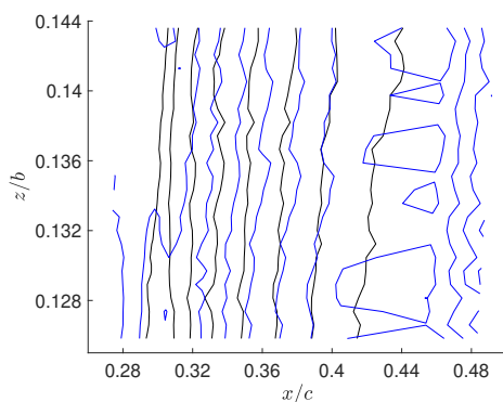
Fig. 5 Contours of U_e/U_\infty within the measurement region for (black) No grid, and (blue) Grid I. Contours levels in range 0.97–1.05 with 0.01 spacing.
