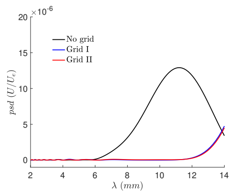
Fig. 9 Spatial psd at x/c = 40\% for the three FST levels.
