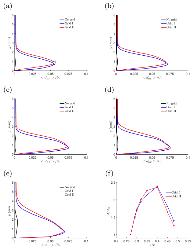
Fig. 11 Unsteady disturbance profiles measured in the CF travelling wave bandpass frequencies ( 80 \text{ Hz} < f < 200 \text{ Hz} ) at x/c = (a) 27%, (b) 29%, (c) 30%, (d) 32%, (e) 35%. (f) Growth of unsteady modes based upon the area within the disturbance profile ( A = 1/\delta \int_0^\delta u'_{BF}/U_e dy ).
