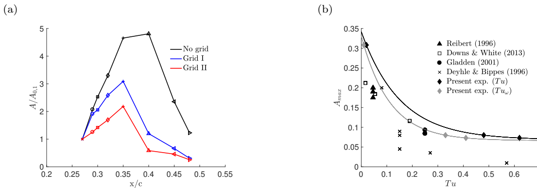
Fig. 8 Growth of primary stationary modes based upon the integral area below the local rms profile ( A_i = 1/\delta_i \int_0^{\delta_i} rms[(U - \bar{U})/U_e] dy ) . Stationary mode saturation amplitude as a function of Tu levels from previous and current work.
