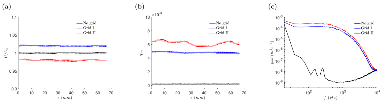
Fig. 4 Spanwise variation of the (a) U/U_e and (b) Tu inside (light) and outside (dark) the boundary layer ( y = 3 mm and y = 6 mm, respectively). (c) Temporal spectra of the fluctuating signals upstream of the model.
