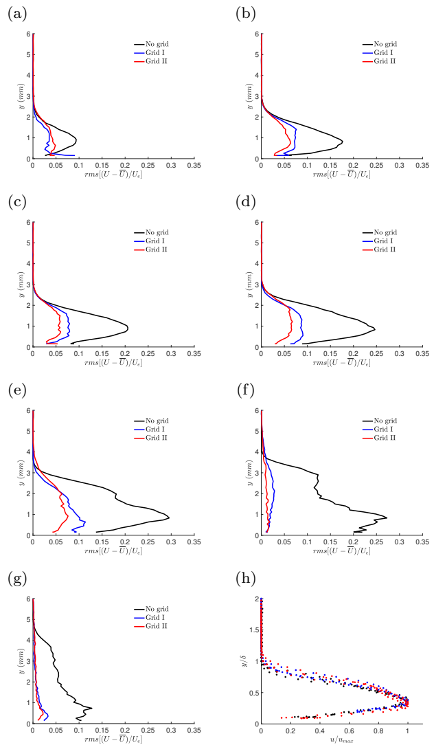
Fig. 7 Amplitude of the primary stationary CF mode at x/c = (a) 27%, (b) 29%, (c) 30%, (d) 32%, (e) 35%, (f) 40%, (g) 45% for the different Tu . (h) Universal shape of the disturbance shape within their linear development (i.e., x/c < 0.35\% ).
