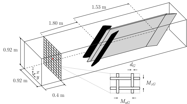
Fig. 1 Schematic of the wind tunnel setup and turbulence screens. Displacement bodies are visible in black, while the flat plate is identifiable in grey. The red dot identifies the origin of the coordinate system, whose principal directions are included at the bottom of the picture for visibility reasons.
