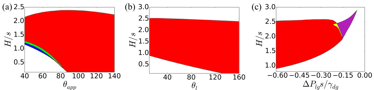
FIG. 4. Morphology phase diagrams for a capillary bridge between two LIS. In panel (a), we vary the apparent contact angle \theta_{app} and normalised separation H/s , and fix the lubricant Neumann angle \theta_l = 160^\circ and normalised lubricant pressure \Delta P_{lg}s/\gamma_{dg} = -0.62 . In panel (b), we vary H/s and \theta_l , keeping \theta_{app} = 100^\circ and \Delta P_{lg}s/\gamma_{dg} = -0.62 . In panel (c), H/s and \Delta P_{lg}s/\gamma_{dg} are varied, with \theta_{app} = 100^\circ and \theta_l = 10^\circ . In all panels, the wetting contact angles for the lubricant are set at \theta_{ld}^{eff} = \theta_{lg}^{eff} = 5^\circ . The red region denotes stable morphologies when the droplet remains attached to both LIS substrates, blue when the droplet is detached from both substrates, and purple when the droplet is detached from one of the substrates. The green and yellow regions in panels (a) and (c) represent regions where multiple morphologies are possible.
