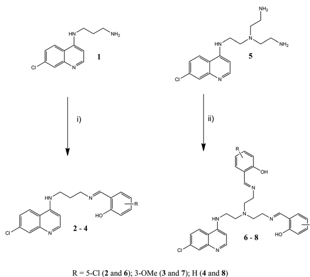
Scheme 1 Synthesis of mono-salicylaldehyde quinoline ligands ( 2–4 ) and bis-salicylaldehyde quinoline ligands ( 6–8 ). (i) appropriate salicylaldehyde (1 eq.), diethyl ether, 16 h, r.t.; (ii) appropriate aldehyde (2 eq.), EtOH, 16 h, r.t.
