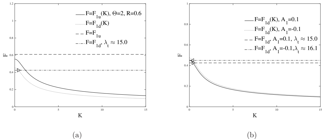
Figure 13. Dispersion relations with (\Theta, R, \beta) = (2, 0.6, 1) and predicted wavenumbers for Regime (II). (a) Theoretical result ( \lambda_t \approx 15.0 ) for the case of Fig. 11c: dispersion curve F_{1u}(K) (solid line), dispersive curve F_{1d}(K) (dotted line), computed upstream Froude number (horizontal dashed line), and computed downstream Froude number (horizontal dash-dotted line). (b) Theoretical result ( \lambda_t \approx 15.0 ) for the solid-line case of Fig. 12: dispersion curve F_{1d}(K) (solid line) and computed downstream Froude number (horizontal dashed line); theoretical result ( \lambda_t \approx 16.1 ) for the dotted-line case of Fig. 12: dispersion curve F_{1d}(K) (dotted line) and computed downstream Froude number (horizontal dash-dotted line).
