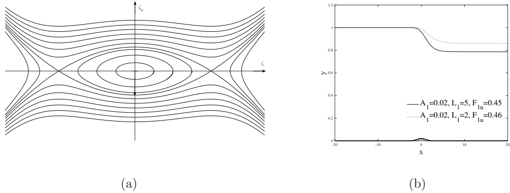
Figure 7. Interfacial hydraulic falls over one obstacle in Regime (IV) with \Theta = \sqrt{3/5} and F_{1u}^* = 0.48 . (a) Phase portrait for the KdV equation with the topography approximated by a positive Dirac delta function. (b) Wave profiles of the full Euler equations for convex obstacles with different widths: A_1 = 0.02 , L_1 = 5 , F_{1u} = 0.45 (solid line); A_1 = 0.02 , L_1 = 2 , F_{1u} = 0.46 (dotted line).
