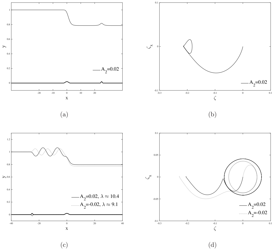
Figure 17. Wave profiles of interfacial hydraulic falls over two successive obstructions and phase portraits in Regime (IV), computed with the full Euler equations with (A_1, L_1, x_1) = (0.02, 5, 0) . Other parameter are: (a, b) (A_2, L_2, x_2) = (0.02, 2, 25) ; (c, d) (A_2, L_2, x_2) = (0.02, 2, -25) , \lambda = 10.4 (solid line) and (A_2, L_2, x_2) = (-0.02, 2, -25) , \lambda = 9.1 (dotted line).
