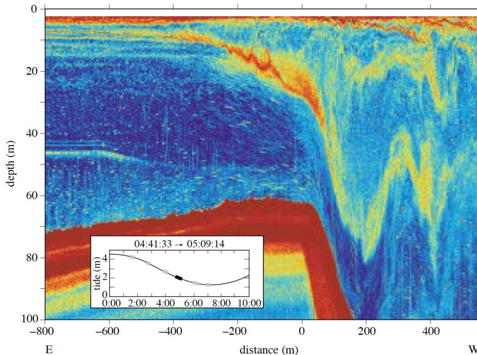
Figure 1. A field observation of internal hydraulic jump obtained by Farmer and Armi near the sill in Knight Inlet in Autumn 1995 (see Figure 7d in [12]).
