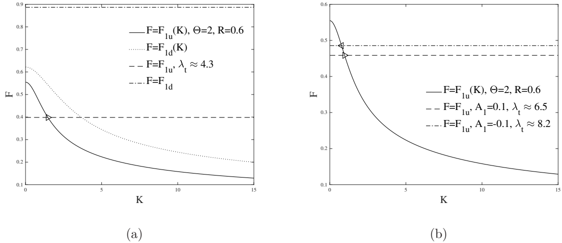
Figure 10. Dispersion relations, F_{1u} (solid lines) and F_{1d} (dotted line) given in Eqs. (11) and (13) with (\Theta, R, \beta) = (2, 0.6, 1) , and predicted wavenumbers for Regime (I). (a) The theoretical prediction of the wavenumber for the solid-line case in Fig. 8c. The obtained upstream Froude number (horizontal dashed line) and downstream Froude number (horizontal dash-dotted line) indicate trapped waves upstream with \lambda_t \approx 4.3 . (b) For the cases in Fig. 9, the computed upstream Froude numbers (horizontal dashed and dash-dotted lines) intersecting the dispersion relation (11) gives the theoretical wavenumbers of trapped waves: \lambda_t \approx 6.5 for (A_1, A_2) = (0.1, -0.1) and \lambda_t \approx 8.2 for (A_1, A_2) = (-0.1, 0.1) .
