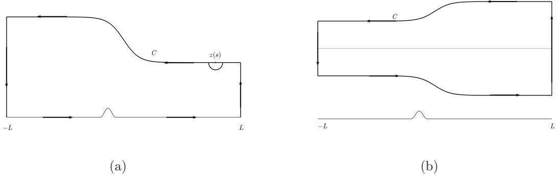
Figure 3. Sketch of the contour of integration: (a) for the lower fluid; (b) for the upper fluid.
