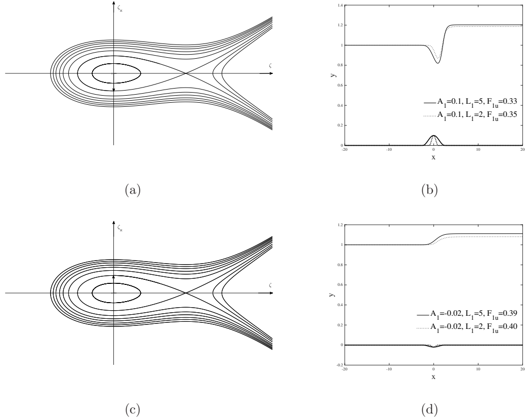
Figure 6. Interfacial hydraulic falls over one obstacle in Regime (III). (a) Phase portrait for the KdV equation with the topography approximated by a positive Dirac delta function. (b) Wave profiles of the full Euler equations for convex obstacles with different widths: A_1 = 0.1 , L_1 = 5 , F_{1u} = 0.33 (solid line); A_1 = 0.1 , L_1 = 2 , F_{1u} = 0.35 (dotted line). (c) Phase portrait for the KdV equation with the topography approximated by a negative Dirac delta function. (d) Wave profiles of the full Euler equations for concave obstacles with different widths: A_1 = -0.02 , L_1 = 5 , F_{1u} = 0.39 (solid line); A_1 = -0.02 , L_1 = 2 , F_{1u} = 0.40 (dotted line).
