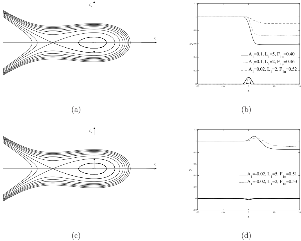
Figure 4. Interfacial hydraulic falls over one obstacle in Regime (I). (a) Phase portrait for the KdV equation with the topography approximated by a positive Dirac delta function. (b) Wave profiles of the full Euler equations for convex obstacles with different sizes: A_1 = 0.1 , L_1 = 5 , F_{1u} = 0.4 (solid line); A_1 = 0.1 , L_1 = 2 , F_{1u} = 0.46 (dotted line); A_1 = 0.02 , L_1 = 2 , F_{1u} = 0.52 (dashed line). (c) Phase portrait for the KdV equation with the topography approximated by a negative Dirac delta function. (d) Wave profiles of the full Euler equations for concave obstacles with different widths: A_1 = -0.02 , L_1 = 5 , F_{1u} = 0.51 (solid line); A_1 = -0.02 , L_1 = 2 , F_{1u} = 0.53 (dotted line).
