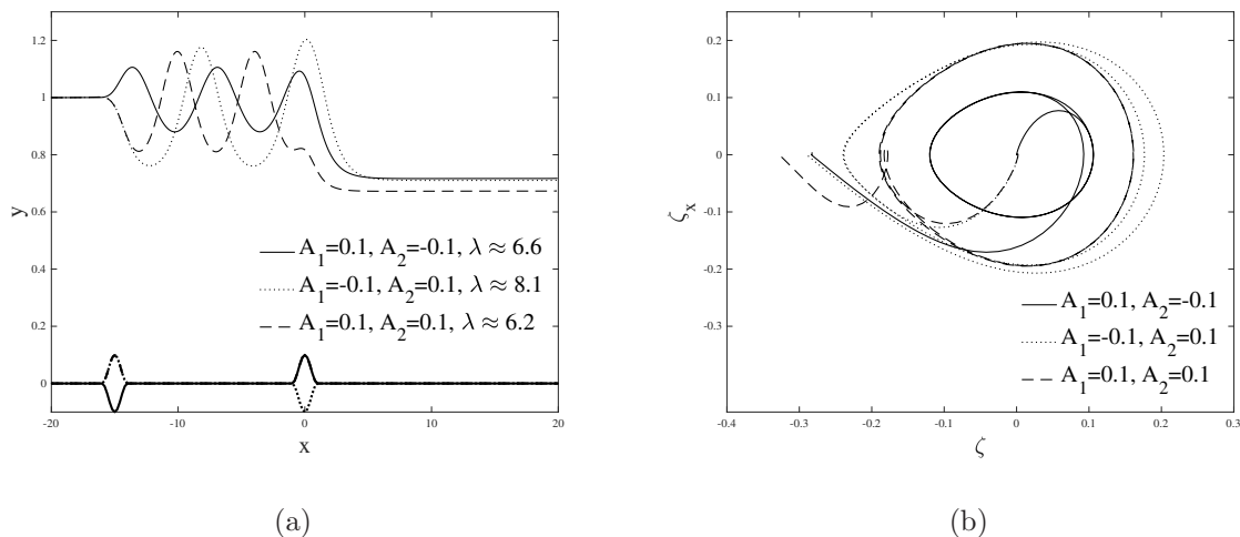
Figure 9. Interfacial hydraulic falls over two successive obstacles of mixed type in Regime (I). The wave profiles (a) and phase portraits (b) are obtained by solving the full Euler equations with L_1 = L_2 = 2 , x_1 = 0 , and x_2 = -15 ; other parameters are: A_1 = 0.1 , A_2 = -0.1 , \lambda \approx 6.6 (solid line); A_1 = -0.1 , A_2 = 0.1 , \lambda \approx 8.1 (dotted line). The numerical results with two successive convex obstacles are presented for comparison and the parameters are A_1 = -0.1 , A_2 = 0.1 , \lambda \approx 6.2 (dashed line).
