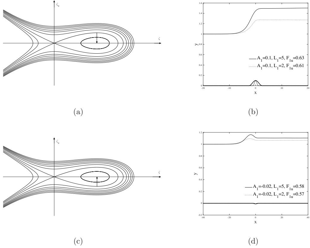
Figure 5. Interfacial hydraulic falls over one obstacle in Regime (II). (a) Phase portrait for the KdV equation with the topography approximated by a positive Dirac delta function. (b) Wave profiles of the full Euler equations for convex obstacles with different widths: A_1 = 0.1 , L_1 = 5 , F_{1u} = 0.63 (solid line); A_1 = 0.1 , L_1 = 2 , F_{1u} = 0.61 (dotted line). (c) Phase portrait for the KdV equation with the topography approximated by a negative Dirac delta function. (d) Wave profiles of the full Euler equations for concave obstacles with different widths: A_1 = -0.02 , L_1 = 5 , F_{1u} = 0.58 (solid line); A_1 = -0.02 , L_1 = 2 , F_{1u} = 0.57 (dotted line).
