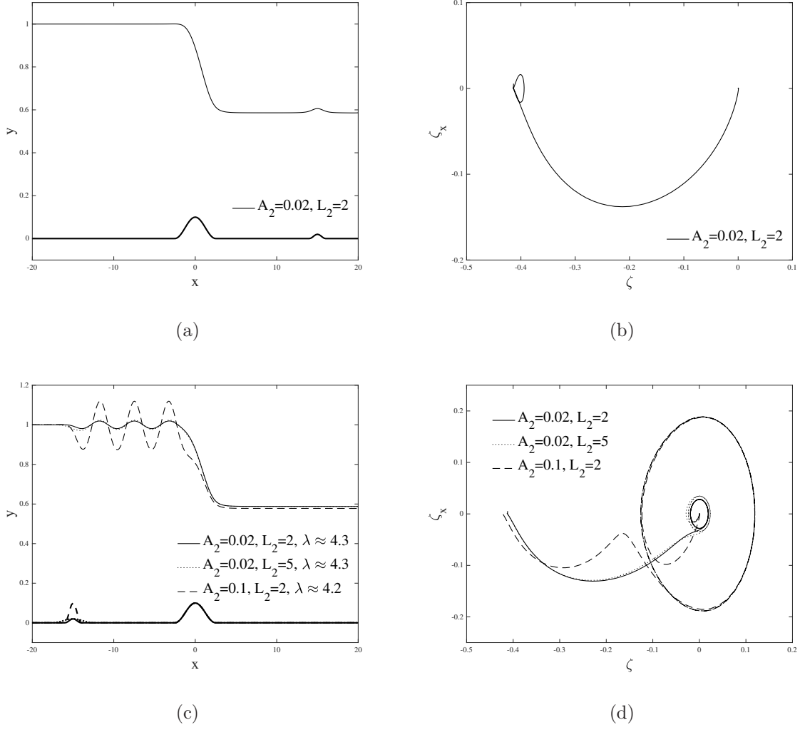
Figure 8. Interfacial hydraulic falls over two convex obstacles in Regime (I) with A_1 = 0.1 , L_1 = 5 , and x_1 = 0 . (a, b) A soliton-like solution and its phase portrait in the full Euler equations with A_2 = 0.02 , L_2 = 2 , and x_2 = 15 . (c, d) Trapped wave solutions and their phase portraits for x_2 = -15 and various aspect ratios of the second obstacle: A_2 = 0.02 , L_2 = 2 , \lambda \approx 4.3 (solid line); A_2 = 0.02 , L_2 = 5 , \lambda \approx 4.3 (dotted line); A_2 = 0.1 , L_2 = 2 , \lambda \approx 4.2 (dashed line).
