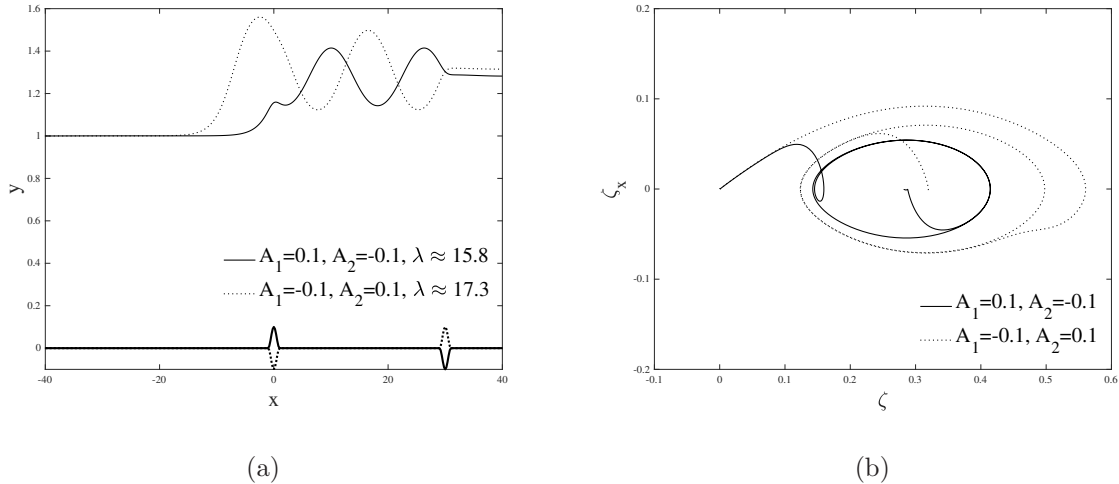
Figure 12. Trapped wave profiles (a) and phase portraits (b) of interfacial hydraulic falls over two successive obstacles of mixed type in Regime (II). Solid lines: (A_1, L_1, x_1) = (0.1, 2, 0) , (A_2, L_2, x_2) = (-0.1, 2, 30) , and \lambda \approx 15.8 ; dotted lines: (A_1, L_1, x_1) = (-0.1, 2, 0) , (A_2, L_2, x_2) = (0.1, 2, 30) , and \lambda \approx 17.3 .
