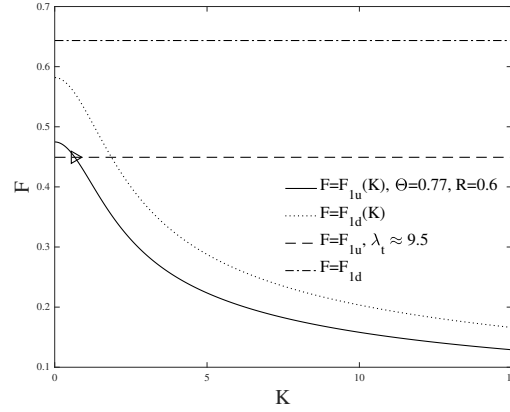
Figure 18. Dispersion relation with (\Theta, R, \beta) = (0.77, 0.6, 1) and predicted wavenumber ( \lambda \approx 9.5 ) for the examples shown in Fig. 17c. Solid line: dispersion relation F_{1u}(K) ; dotted line: dispersion relation F_{1d}(K) ; horizontal dashed line: computed upstream Froude number; horizontal dash-dotted line: computed downstream Froude number.
