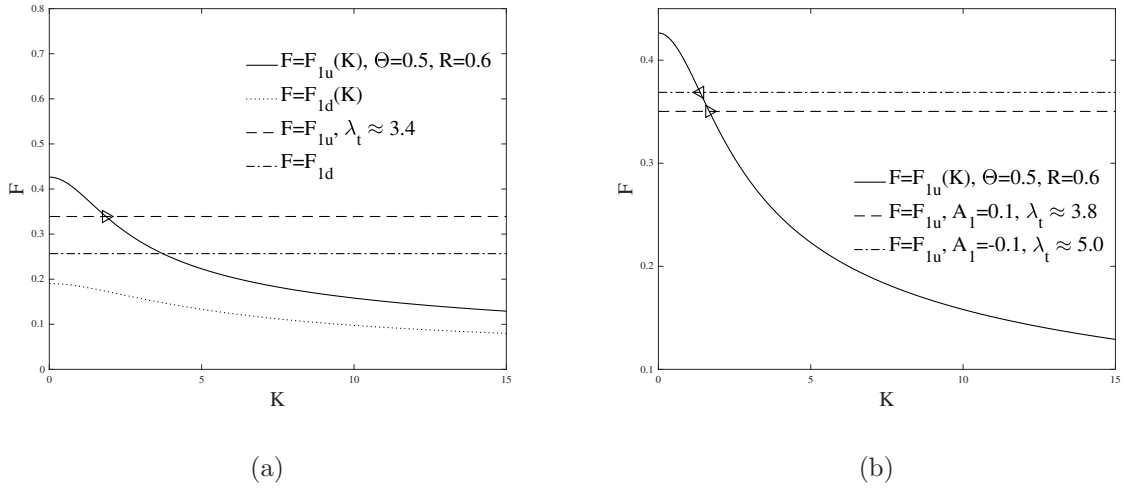
Figure 16. Dispersion relations with (\Theta, R, \beta) = (0.5, 0.6, 1) and predicted wavenumbers for Regime (III). (a) Theoretical result ( \lambda_t \approx 3.4 ) for the solid-line case of Fig. 14c: dispersion curve F_{1u}(K) (solid line), dispersion curve F_{1d}(K) (dotted line), computed upstream Froude number (horizontal dashed line), and computed downstream Froude number (horizontal dash-dotted line). (b) Theoretical predictions of wavenumber for the examples shown in Fig. 15: \lambda_t \approx 3.8 for the case A_1 = 0.1 and \lambda_t \approx 5.0 for the case A_1 = -0.1 . Solid line: dispersion curve F_{1u}(K) ; horizontal dashed line: computed upstream Froude number for the case A_1 = 0.1 ; horizontal dash-dotted line: computed upstream Froude number for the case A_1 = -0.1 .
