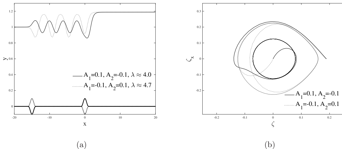
Figure 15. Trapped wave profiles (a) and phase portraits (b) of interfacial hydraulic falls over two successive obstacles of mixed type in Regime (XXIII). Solid lines: (A_1, L_1, x_1) = (0.1, 2, 0) , (A_2, L_2, x_2) = (-0.1, 2, -15) , and \lambda \approx 4.0 ; dotted lines: (A_1, L_1, x_1) = (-0.1, 2, 0) , (A_2, L_2, x_2) = (0.1, 2, -15) , and \lambda \approx 4.7 .
