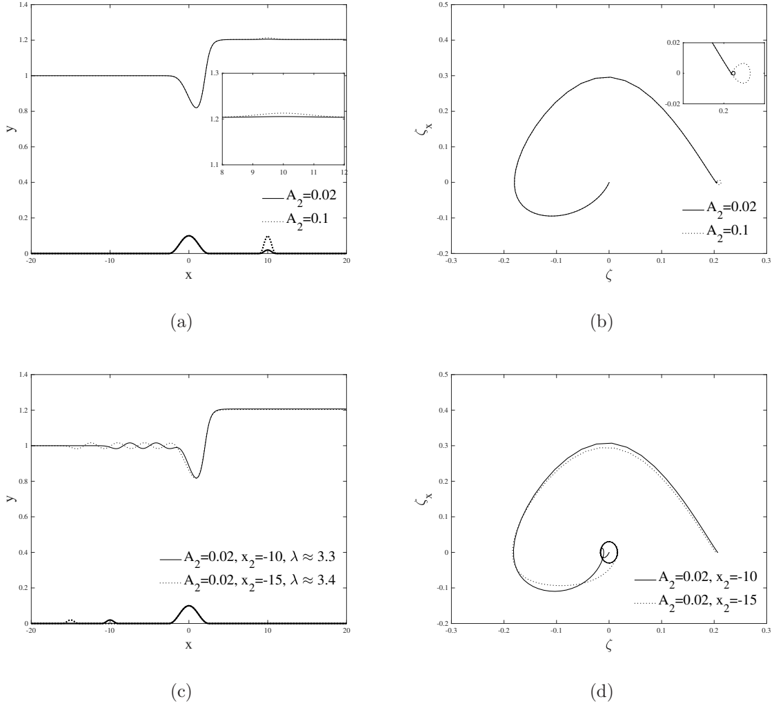
Figure 14. Wave profiles of interfacial hydraulic falls over two successive convex obstructions and phase portraits in Regime (III), computed with the full Euler equations with (A_1, L_1, x_1) = (0.1, 5, 0) and L_2 = 2 . Other parameter are: (a, b) A_2 = 0.02, x_2 = 10 (solid line) and A_2 = 0.1, x_2 = 10 (dotted line); (c, d) A_2 = 0.02, x_2 = -10, \lambda \approx 3.3 (solid line) and A_2 = 0.02, x_2 = -15, \lambda \approx 3.4 (dotted line).
