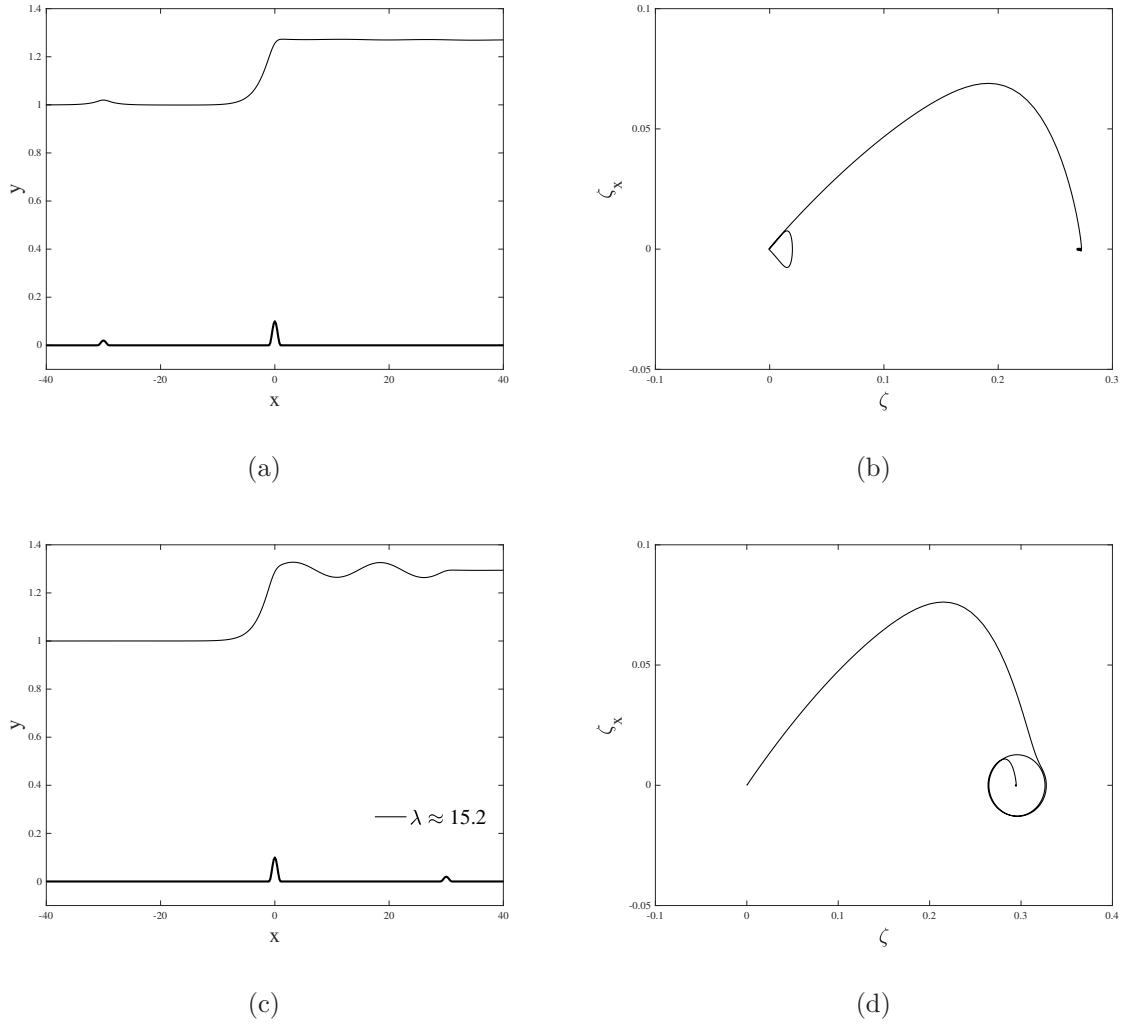
Figure 11. Interfacial hydraulic falls over two successive convex obstacles in Regime (II), computed in the full Euler equations with (A_1, L_1, x_1) = (0.1, 2, 0) and (A_2, L_2, x_2) = (0.02, 2, \pm 30) . (a, b) Wave profile and phase portrait for x_2 = -30 . (c, d) Wave profile and phase portrait for x_2 = 30 , exhibiting trapped waves downstream with \lambda \approx 15.2 .
