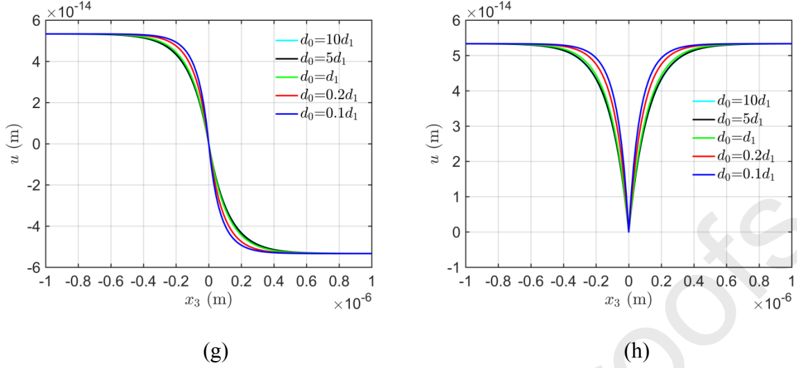
Fig. 3. Electromechanical fields for different diameters at the interface. (a), (c), (e), and (g) are respectively the electric potential function \varphi , electric field E_3 , strain S_3 , and mechanical displacement u_3 for a uniform c -axis, and (b), (d), (f) and (h) are those fields for an opposite c -axis.
