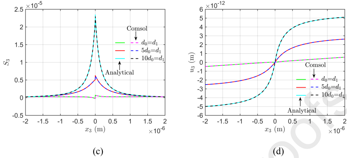
Fig. A. Comparisons of linear analytical and nonlinear numerical solutions at a heterogeneous junction for F = 1 nN: (a) Electric potential \phi , (b) Electric field E_3 , (c) Strain S_3 , and (d) Mechanical displacement u_3 .
