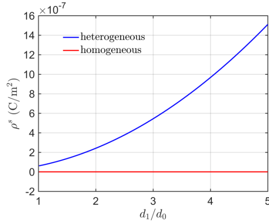
Fig. 6 Interface polarization charge density \rho^s versus the diameter ratio d_1/d_0
