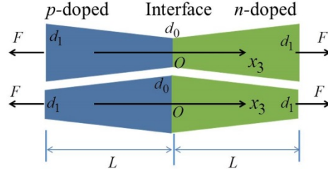
Fig. 1. Sketch of non-uniform PS PN junctions
