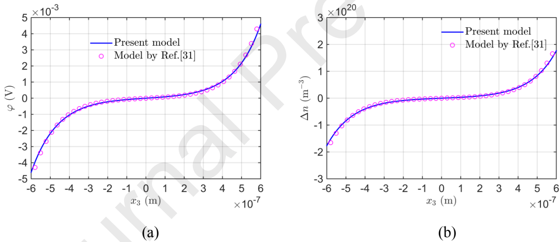
Fig. 2. A comparison of the present results with the results in Ref. [31]. (a) Electric potential function, (b) Electron concentration perturbation.
