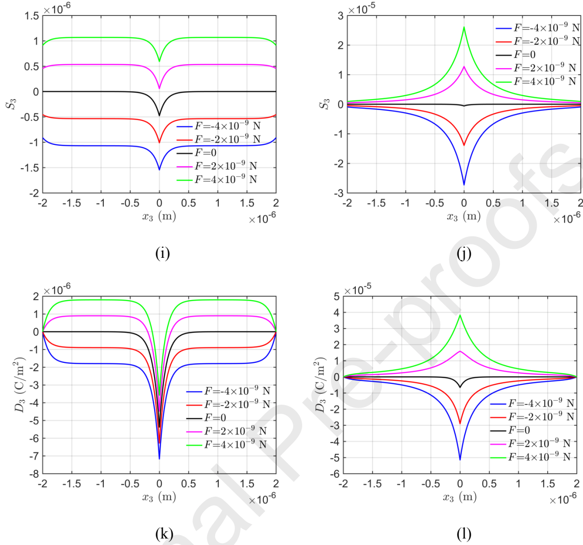
Fig. 4. Electromechanical fields of homogeneous PS PN junctions for different values of F . (a), (c), (e), (g), (i) and (k) respectively stand for the distributions of the electric potential function \varphi , electric field E_3 , electron concentration n , hole concentration p , strain S_3 , and electric displacement D_3 of a uniform PN junction with a constant cross section, and (b), (d), (f), (h), (j) and (l) are those fields for the case of a variable cross section.
