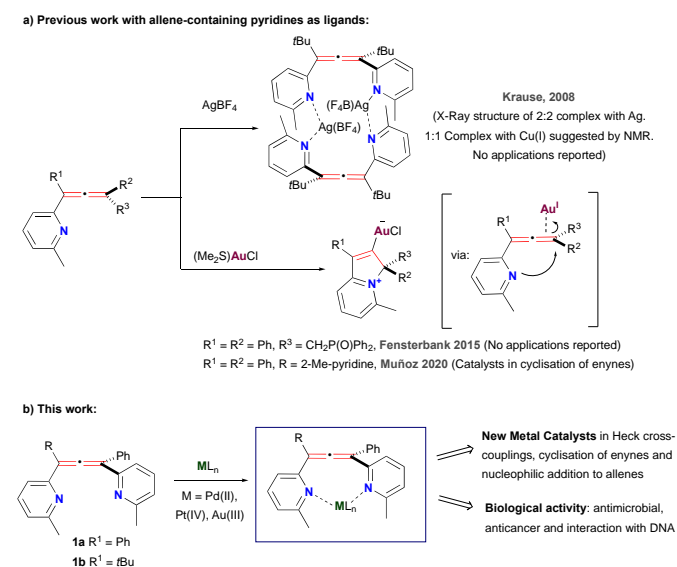
Figure 3. Previous (a) and present (b) work with allene-containing pyridines as ligands.
