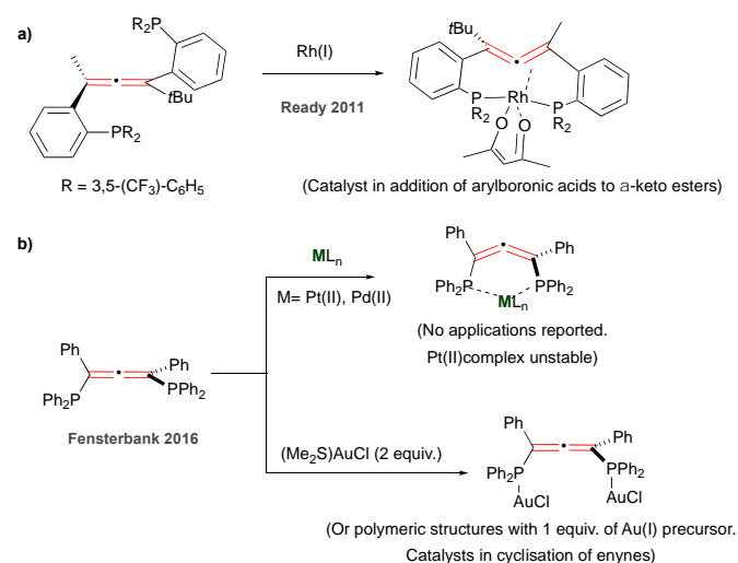
Figure 2. Previous work with allene-containing phosphines as ligands.
