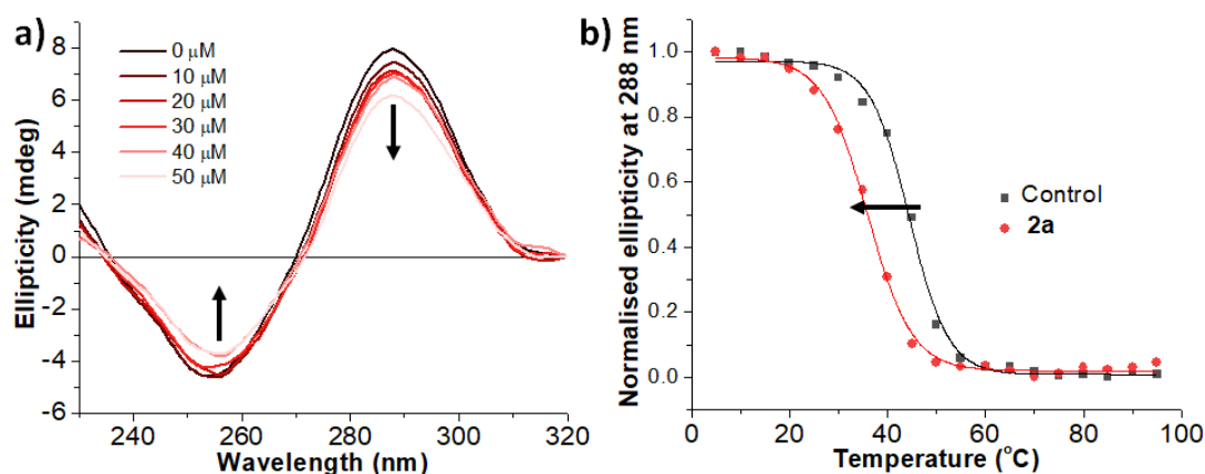
Figure 4. Interaction of compound 2a with i-motif DNA. A) Circular dichroism spectroscopy of hTeloC (10 \mu\text{M} ) in 10 mM sodium cacodylate buffer, 100 mM KCl, pH 5.5. 0-5 equiv. of compound 2a . B) CD melting experiment with hTeloC in the absence (black) and in the presence of 5 equiv. of compound 2a (red).
