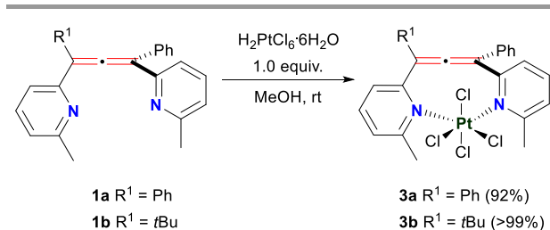
Scheme 2. Synthesis of Pt(IV)-complexes 3a-b .
