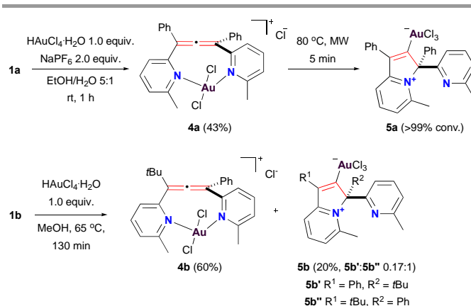
Scheme 3. Synthesis of Au(III)-complexes 4a-b and 5a-b .
