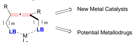
Figure 1. Different types of interaction of allene frameworks with metals.
