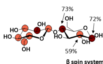
Figure 4. Effect of phosphate on the binding of D-cellobiose to CDP. Binding epitope mappings derived from the initial slope approach for each isolated proton. [13] a) sample in 25 mM [D_{11}]\text{Tris} pH 7.4, 100 mM NaCl in the presence of 100 \mu\text{M} \text{K}_3\text{PO}_4 , and b) sample in 25 mM PBS pH 7.4, isotonic. The maximum \text{STD}_0 was observed for H2 in the non-reducing ring, to which an arbitrary value of 100% was assigned. The \text{STD}_0 of the other protons were normalised against H2.
