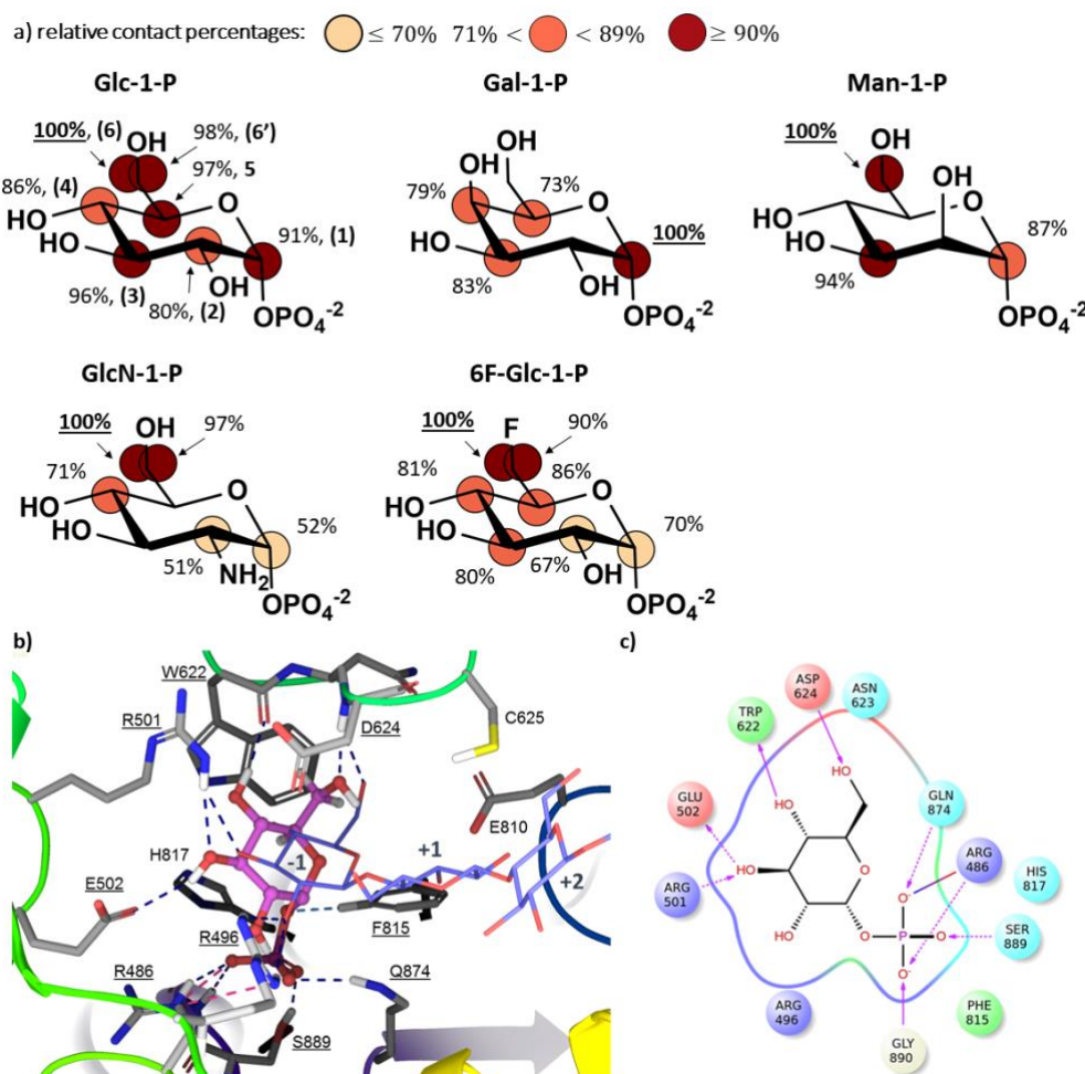
Figure 1. Molecular recognition of natural and non-natural donor-like ligands by CDP a) Binding epitope mappings from STD NMR for the interactions of CDP with the donor substrate Glc-1-P as well as with the non-natural ligands Gal-1-P, Man-1-P, GlcN-1-P and 6F-Glc-1-P. STD NMR experiments were carried out with samples containing 1:200 “binding site to ligand ratio” for Glc-1-P, and 1:100 ratio for Gal-1-P, Man-1-P, GlcN-1-P and 6F-Glc-1-P. All the experiments were carried at 800 MHz and 278 K in [D_{11}] Tris 25 mM, pH 7.4 (NaCl 100 mM). Glucopyranose atoms are numbered in Glc-1-P (top left). b) 3D docking model of the CDP/Glc-1-P complex. The cellotetraose complex (PDB ID 5NZ8, purple wire representation) [11] is superimposed for comparison. For simplicity, only three rings of cellotetraose are shown (sites -1, +1 and +2). Glc-1-P is represented in pink ball-and-sticks and interacting CDP side chains as thick tubes. Non-bonded interactions are in dash-lines; H-bonds are in blue and salt bridges in magenta. c) Ligand interactions diagram of Glc-1-P in the donor binding subsite (-1) of CDP. Arrows indicate donor-to-acceptor H-bonds, dash lines H-bonds with side chains, and solid lines H-bonds with enzyme backbone. The solid line shaded red to blue represents a salt bridge.
