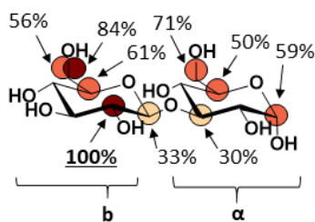
Figure 2. Molecular recognition of natural and non-natural acceptor-like ligands by CDP. Binding epitope mappings from STD NMR for the interactions of CDP with a) D-cellobiose, b) D-cellotriose and c) D-laminaribiose. Numbering of the glucopyranose atom positions is reported in D-cellobiose reducing ring, while the curly brackets below the structures indicate the ring labels. STD NMR experiments were carried out at 800 MHz with samples containing 3 mM ligand and 15 \mu M enzyme binding sites in [D 11 ]Tris 25 mM, pH 7.4 (NaCl 100 mM) at 278 K. Except for all glucose reducing rings and H1 of the non-reducing ring of D-laminaribiose, the STD values reported are average values for both \alpha - and \beta -anomeric forms of the oligosaccharides.
