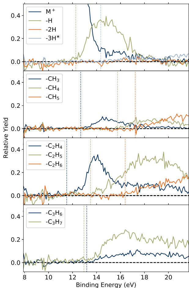
Figure 8. PEPICO yields for n\text{H} - and C_m\text{H}_n -loss from 6H-Pyr. Vertical dotted lines indicate AE_{PEP} . *See the discussion of possible peak-blending in Section 3.1.1
