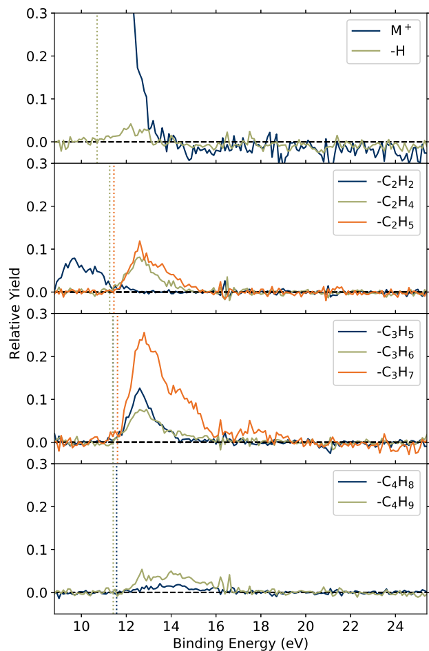
Figure 9. PEPICO yields for H- and C_m\text{H}_n -loss from 16H-Pyr. Vertical dotted lines indicate AE_{PEP} . Note that there are several additional fragmentation channels open in this energy range (see Figure 4) which are not plotted. The total relative yield of the channels shown here is thus less than unity.
