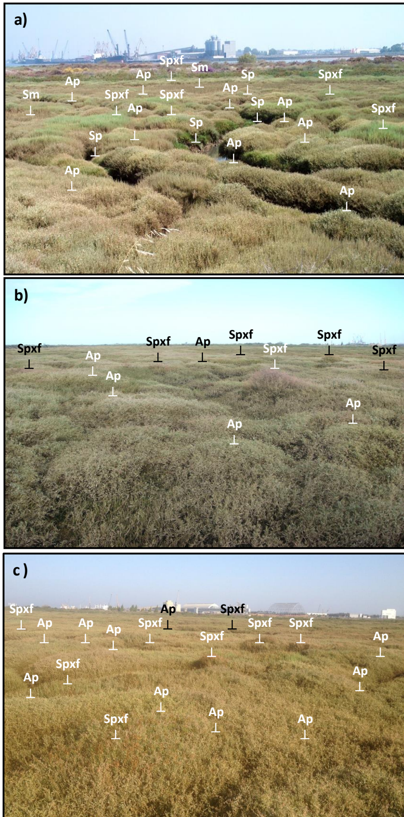
FIGURE S2 Photographs of Don Claudio intertidal lagoon (southwestern Iberian Peninsula) in (a) 2003, (b) 2010 and (c) 2015. Spartina maritima (Sm); Sarcocornia perennis (Sp); S. perennis × fruticosa (Spxf); Atriplex portulacoides (Ap).
