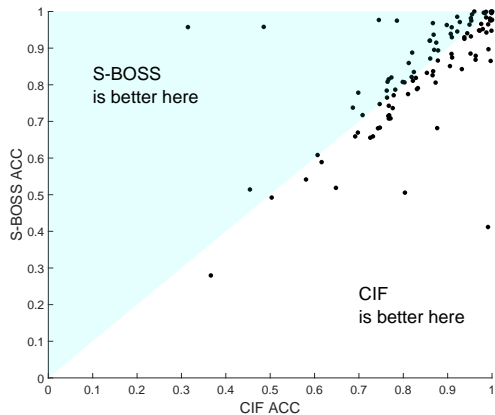
Fig. 6. Scatter plot of S-BOSS and CIF. CIF wins on 59 problems, ties on 1, and loses on 47 problems.
