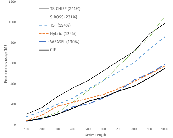
Fig. 11. Memory usage of six classifiers for varying series length. Figures in brackets are the overall percentage of memory used in comparison to CIF.
