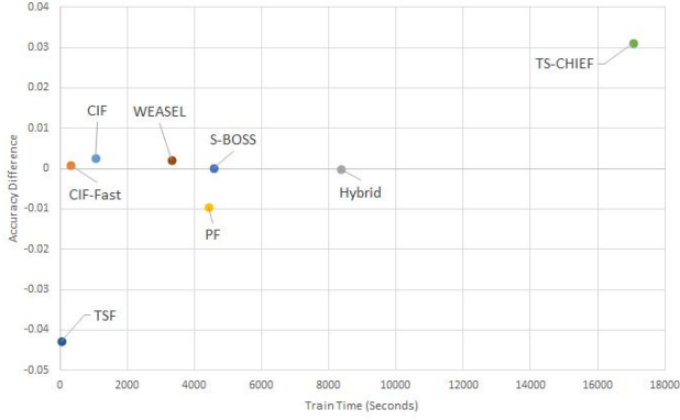
Fig. 10. A comparison of classifiers in terms of accuracy and train time. The y-axis shows the average difference in accuracy from the default hybrid approach. Time and accuracy are averaged over 104 UCR problems.
