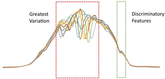
Fig. 1. Time series from the EthanolLevel dataset. While the middle portion (visible light wavelengths) contains the greatest variation, a particular interval (into the near infrared) contains the most discriminatory information for ethanol concentration. An interval-based classifier may be able to compensate for the confounding effect of the visible spectrum.
