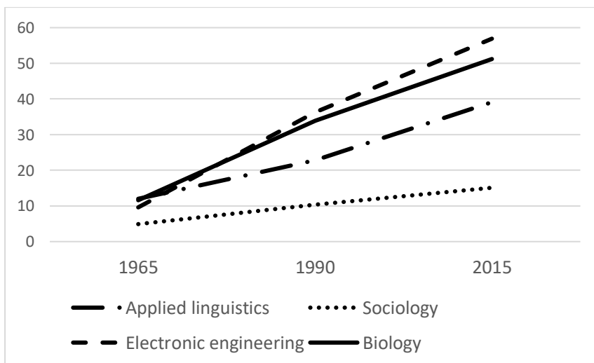
Figure 3: Changes in Use of Acronyms by Discipline (per 10,000 Words)
