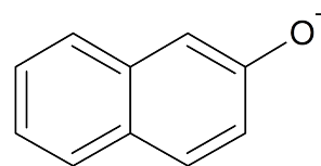
Fig. 1 Structure of 2-naphthoxide, 2-Np − .
