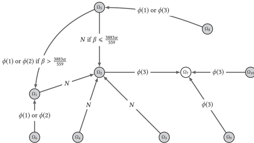
FIGURE 1 Incentivised transitions for (379/523)\alpha_2 < \alpha_1 < \alpha_2
