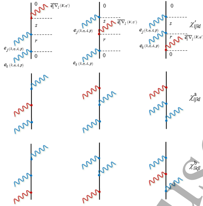
Figure 3: Nine (three sets of three grouped horizontally) topologically distinct Feynman diagrams needed in the calculation of (6). Diagrams to be interpreted the same as in Figure 2, except red wavy lines represent E2 photon couplings to the molecule. Each set of three horizontal Feynman pathways produce the respective polarizability tensor \chi in equations (7) and (8) shown to the right.
