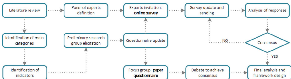
Fig. 1. Delphi consultation methodology.
