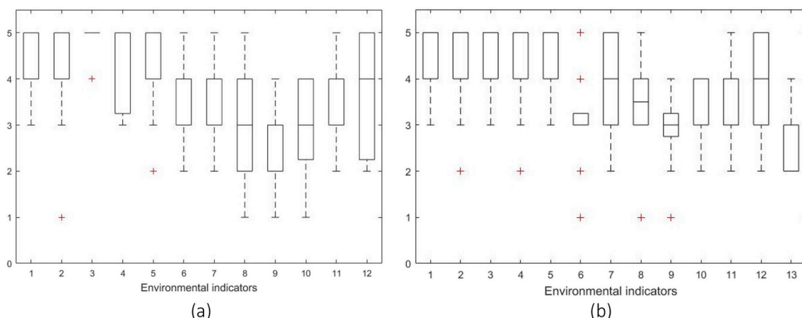
Fig. 2. Environmental boxplots after the first (a) and second (b) rounds of consultation.
