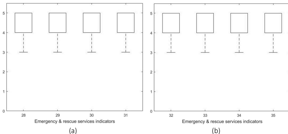
Fig. 6. Emergency & rescue services boxplots after the first (a) and second (b) rounds of consultation.
