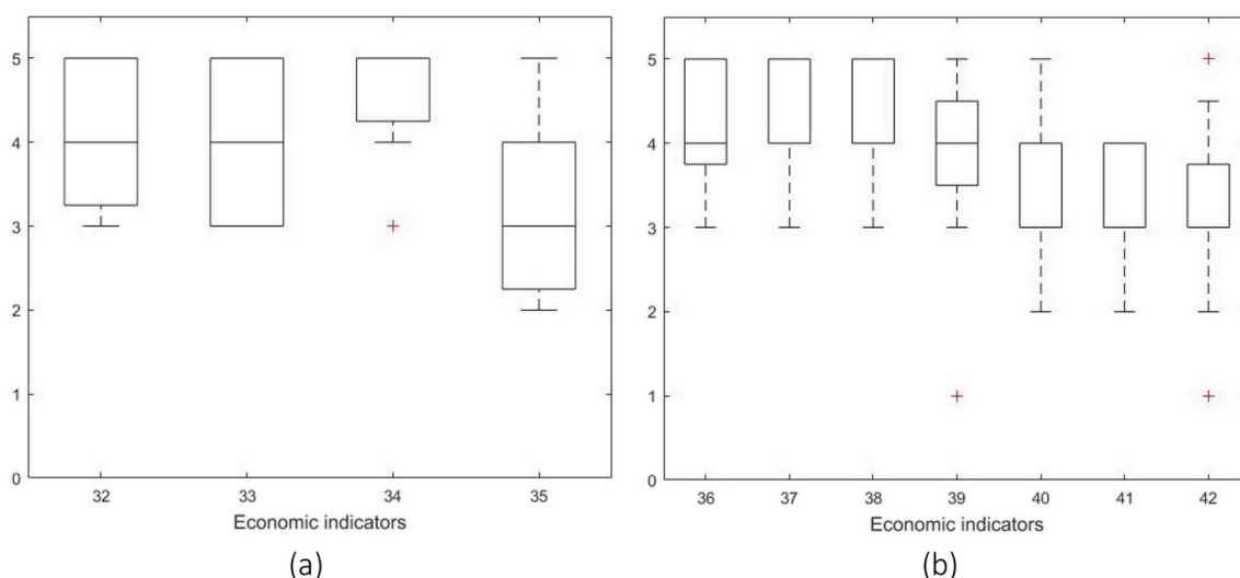
Fig. 7. Economy category boxplots after the first (a) and second (b) rounds of consultation.
