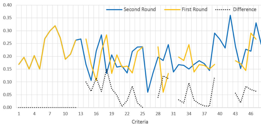
Fig. 9. Variation coefficients for the criteria over the two rounds of consultation.
