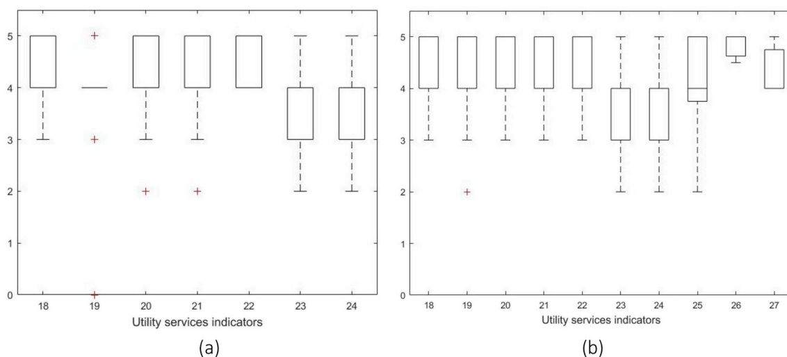
Fig. 4. Utility services boxplots after the first (a) and second (b) rounds of consultation.
