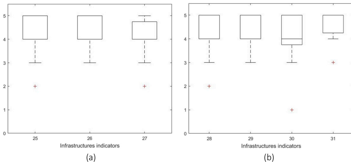
Fig. 5. Infrastructures boxplots after the first (a) and second (b) rounds of consultation.
