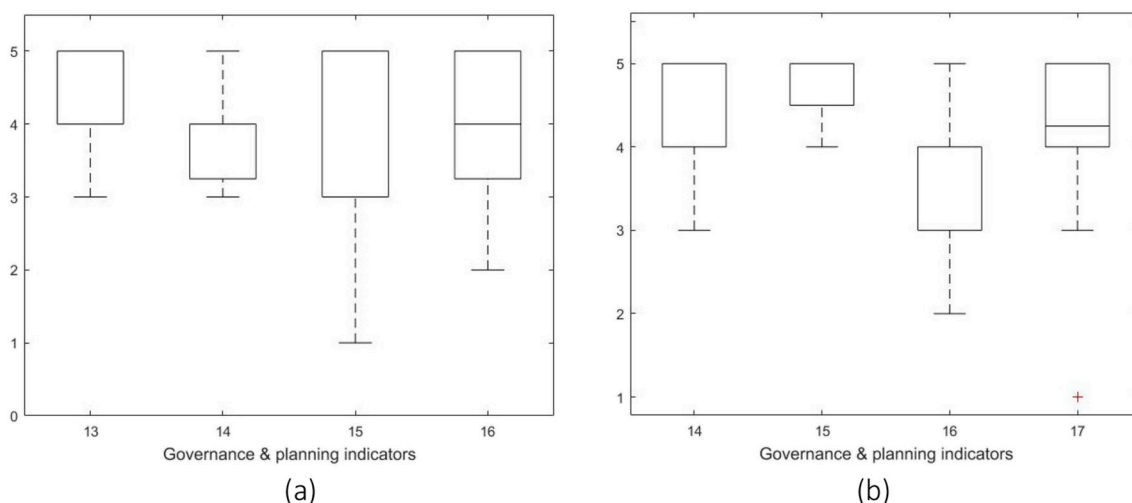
Fig. 3. Governance & planning boxplots after the first (a) and second (b) rounds of consultation.
