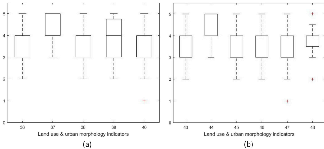
Fig. 8. Land use & urban morphology boxplots after the first (a) and second (b) rounds of consultation.
