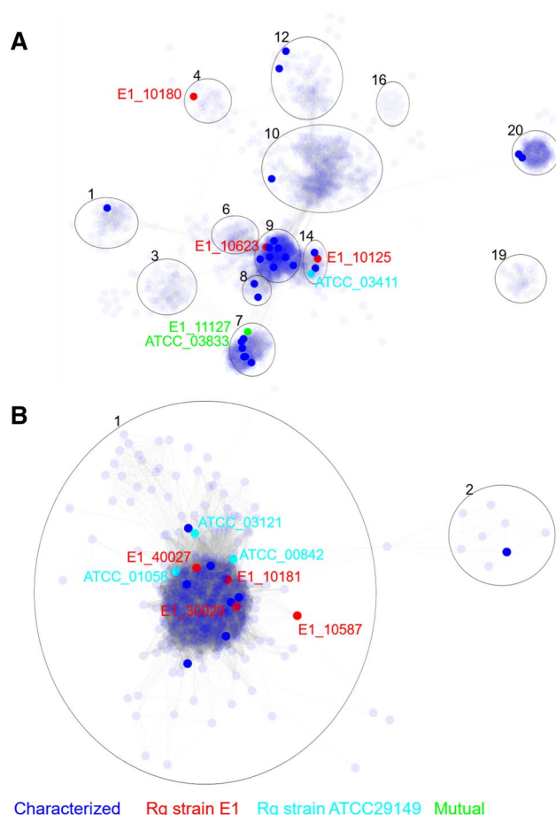
Fig. 2 The distribution of R. gnavus GH29 and GH95 fucosidases based on SSN analysis. a Partial representation of SSN analysis of GH29 family containing fucosidases from R. gnavus E1 and ATCC29149 strains. b Representation of the SSN central cluster of GH95 family containing all GH95 from R. gnavus E1 and ATCC29149 strains. Blue node: sequences extracted from the CAZy database encoding functionally characterized enzymes. Red nodes sequences from R. gnavus E1 strain. Cyan nodes, sequences from R. gnavus ATCC29149 strain. Green nodes, sequences common to both R. gnavus E1 and ATCC29149 strains
