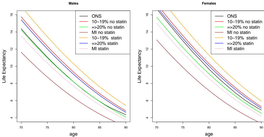
Figure 3: Life expectancy by cardiac risk group with and without statins for ages 70 – 90 based on the ONS period life table centered at 2010 (black line) for males and females.
