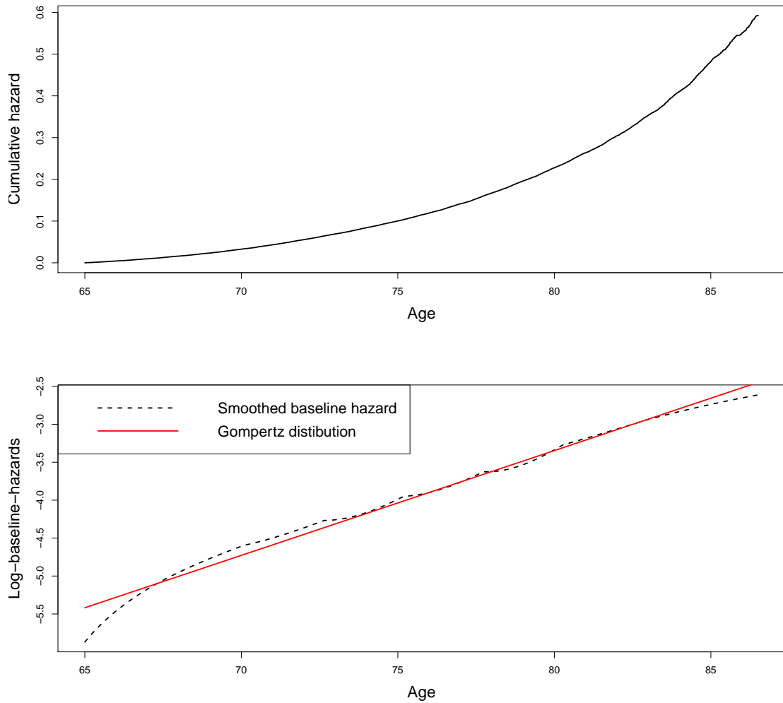
Figure 2: Top: estimated baseline cumulative hazard function \hat{M}_0(t) . Bottom: smoothed baseline hazard \hat{\mu}_0(t) (black) and fitted linear regression line (red) for the statins survival study. Time is age in years.
