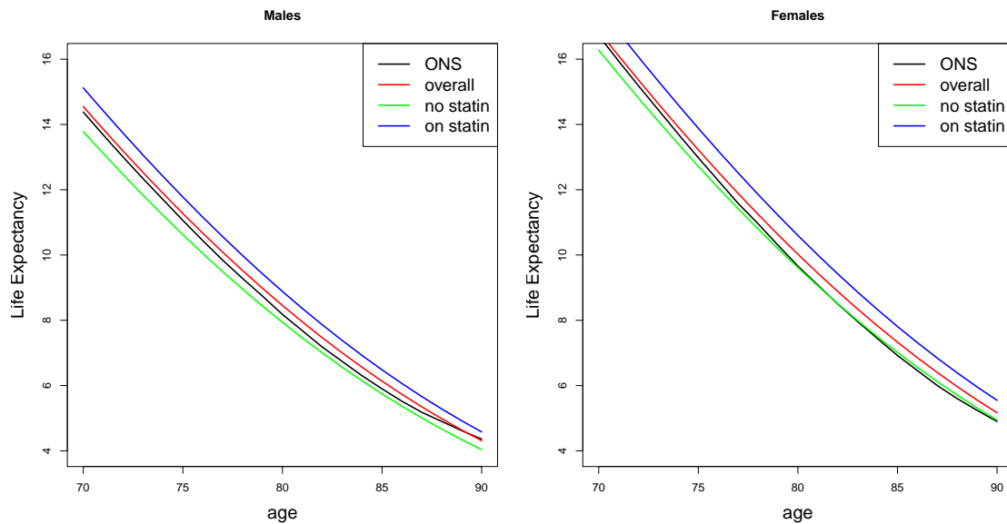
Figure 4: Life expectancy from the ONS period life table centered at 2010 (black line), estimated LEs with/without statins (blue and green lines, respectively), and the combined as in Equation (7) overall population life expectancy (red line) for males and females. (Gompertz parameters were fitted at age 70.)
