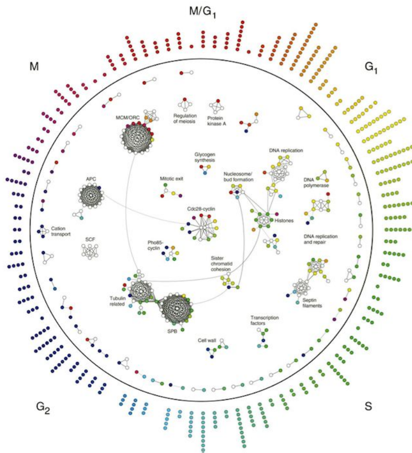
Figure 4. Protein-protein interaction networks in yeast identified by de Lichtenberg et al. (2005). The color-coding represents the period in the cell cycle in which specific proteins are synthesized.
