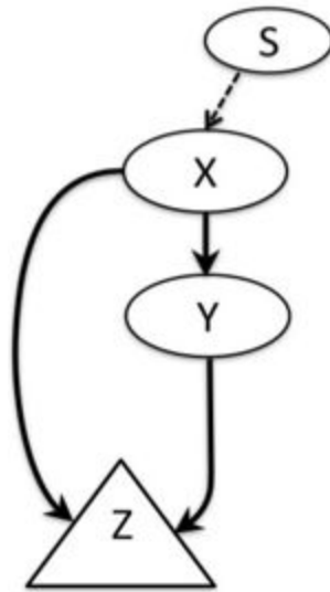
Figure 1. Example of a motifs. A coherent feedforward loop of the sort investigated by Alon.
