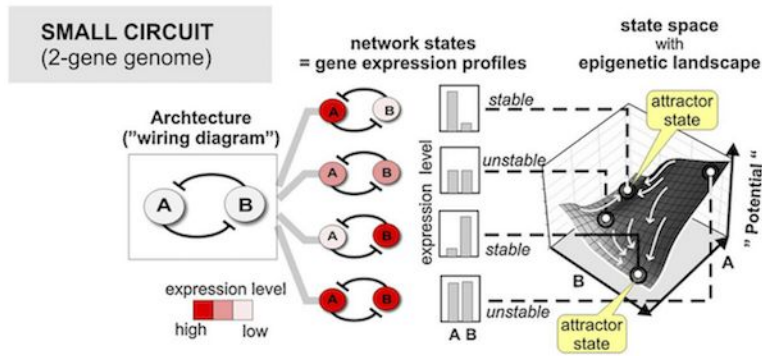
Figure 6. The possible trajectories of a double-negative feedback network between two genes are plotted on a landscape. It has two attractors (stable states of network activity), where some unstable states are also shown. From Huang et al., 2009.
