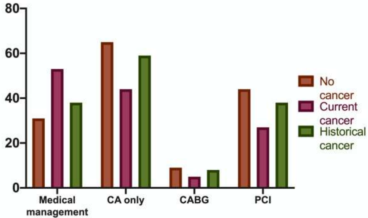
Figure 3: Distribution of treatments among current, historical and no cancer diagnoses
