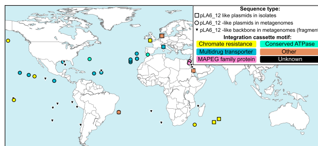
Fig. 3. Biogeography of pLA6_12-like plasmids. Sampling locations of Roseobacter group isolates are shown in squares. Locations where metagenomes have been obtained are shown in circles and triangles. Integration cassette motifs are indicated by a color code consistent with Fig. 2. pLA6_12-like plasmids were found exclusively in marine environments, but scattered across the world. Black triangles represent metagenome fragments, which encode pLA6_12-like repL genes, but are too incomplete to allow conclusions on the respective integration cassette.
