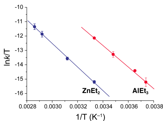
Figure 3. Eyring plots for the ethylation of \mathbf{1Me}_2 with \text{ZnEt}_2 and \text{AlEt}_3 in toluene- d_8 .
