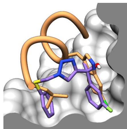
Figure 3. Binding pose of 4 (purple) to hDM2 in the p53 binding site determined by CORCEMA-ST, with an overlay of peptide 1 (orange) showing the binding residues of Leu and Cl-Trp. The surface of hDM2 is cut along the plane of the centroid of the aromatic rings of compound 4 .
