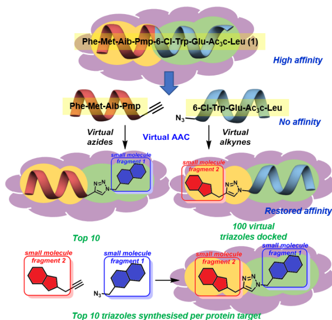
Figure 1. Concept of peptide directed binding utilised in this work with in silico methods to improve the rapid and economic nature of finding new PPI modulators. Peptide 1 binds to hDM2/X , and is separated in to two smaller peptides with no appreciable binding despite having two key residues each. Azide-alkyne cycloaddition (AAC) identifies small molecule fragments which restore binding affinity. The identified small molecule fragments can be combined to generate a small molecule substitute for the initial peptide.
