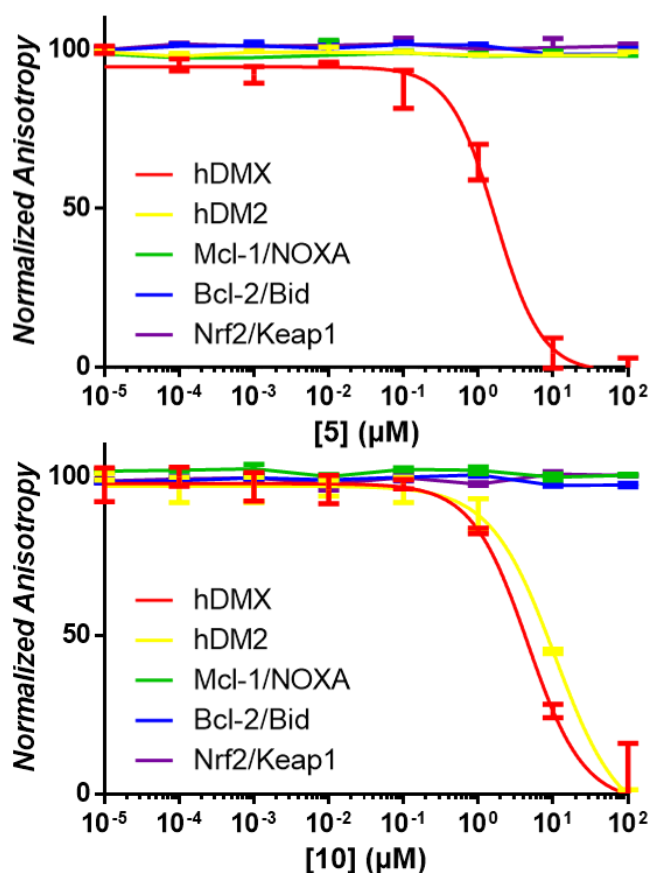
Figure 2. Examples of competitive-displacement assays of small molecules towards a selection of PPIs. Compounds 5 and 10 used to exemplify the titration of compounds towards the hDMX/p53 , hDM2/p53 , Mcl-1/NOXA , Bcl-2/Bid and Nrf2/Keap1 interactions. Dose response curves can be seen for 5 towards hDMX , and for 10 towards hDMX and hDM2 , with no competitive binding towards any other PPIs observed.
