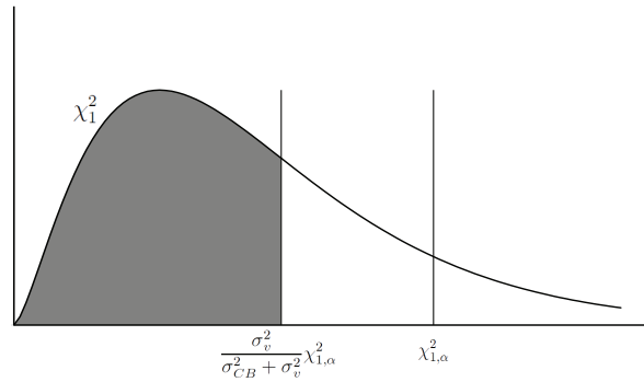
Figure 1: \chi^2 Distribution
