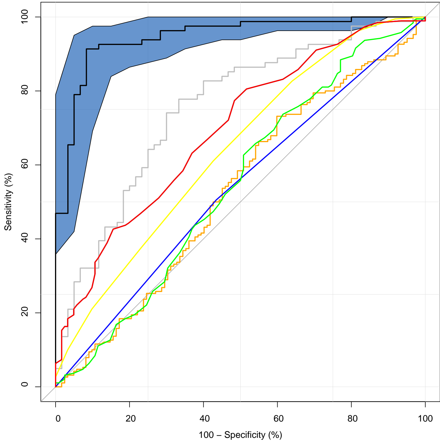
Confidence intervals
