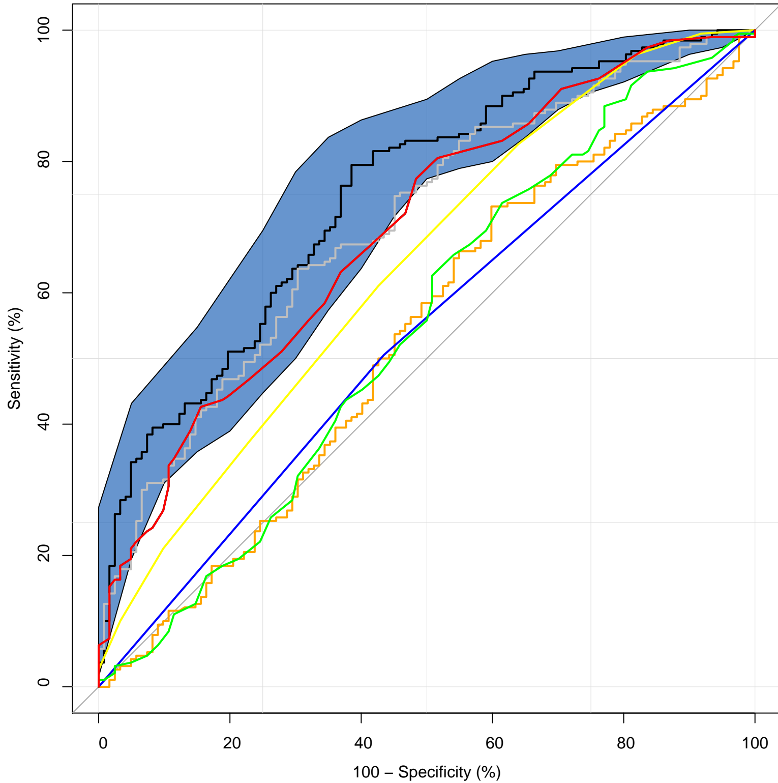
Confidence intervals
