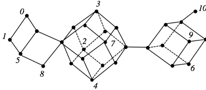
Figure 1: An example of the 1-skeleton of the tight-span of a totally split-decomposable metric defined on the set \{0, 1, 2, \dots, 9, 10\} (the metric is defined in the next section). It is a polytopal complex consisting of 5 blocks: two 1-cubes, a 3-cube, a rhombic dodecahedron and a pair of 2-cubes with an edge in common.
