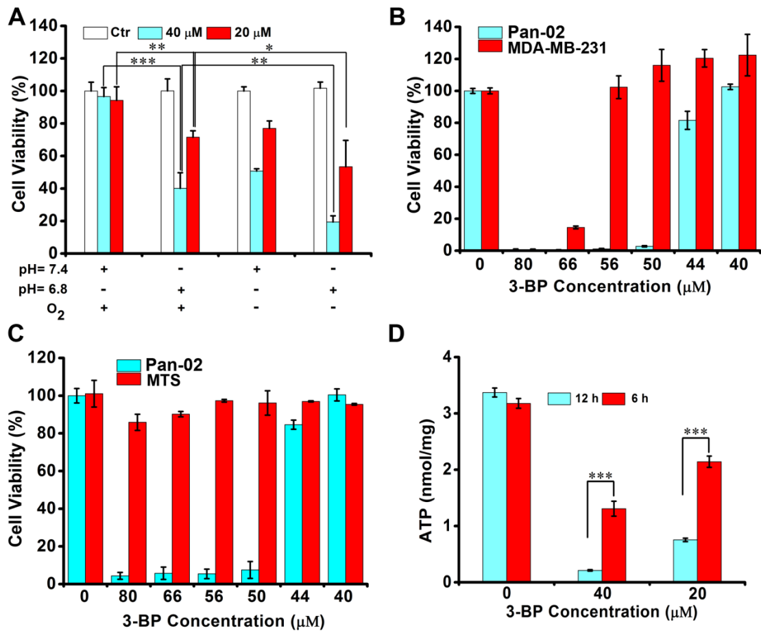
Figure 3. Effects of T-Lipo-3BP on cell viability and ATP production. (A) Viability of Pan-02 tumor cells after treatment with T-Lipo-3BP containing 40 \mu\text{M} or 20 \mu\text{M} 3-BP under both normoxic and hypoxic conditions at pH 7.4 and 6.8 at 37°C for 24 h. * p < 0.05 , ** p < 0.01 , *** p < 0.001 . Error bars represent the mean \pm s.d. of three independent experiments. (B) Cytotoxicity of T-Lipo-3BP containing different concentrations of 3-BP in Pan-02 and MDA-MB-231 tumor cell lines after 24 h of treatment at pH 7.4 under hypoxic conditions. (C) Cytotoxicity of T-Lipo-3BP containing different concentrations of 3-BP in Pan-02 tumor cells and MTS cells after 24 h of treatment at pH 7.4 under hypoxic conditions. (D) Cellular levels of ATP after treatment of Pan-02 cells with different concentrations of 3-BP in T-Lipo-3BP. Error bars represent the mean \pm s.d. of three independent experiments, *** p < 0.001 .
