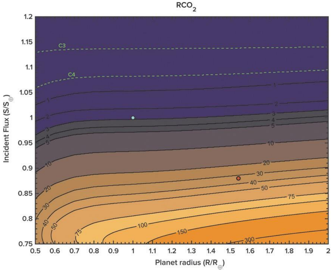
FIG. 5. Contours of atmospheric \text{CO}_2 , in preindustrial units (where 1 \text{ RCO}_2 = 280 \text{ ppm} ), as a function of planet radius (in Earth-relative units) and incident flux (relative to present-day Earth). Also displayed are the C3 and C4 photosynthesis limits.
