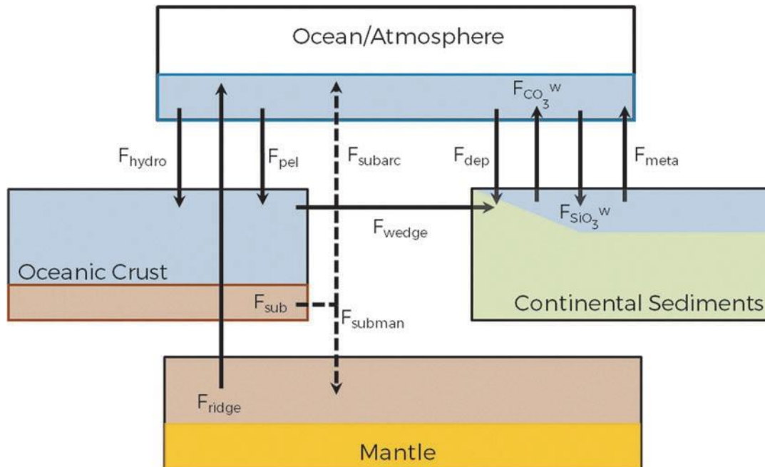
FIG. 1. Model schematic illustrating carbon reservoirs and fluxes.
