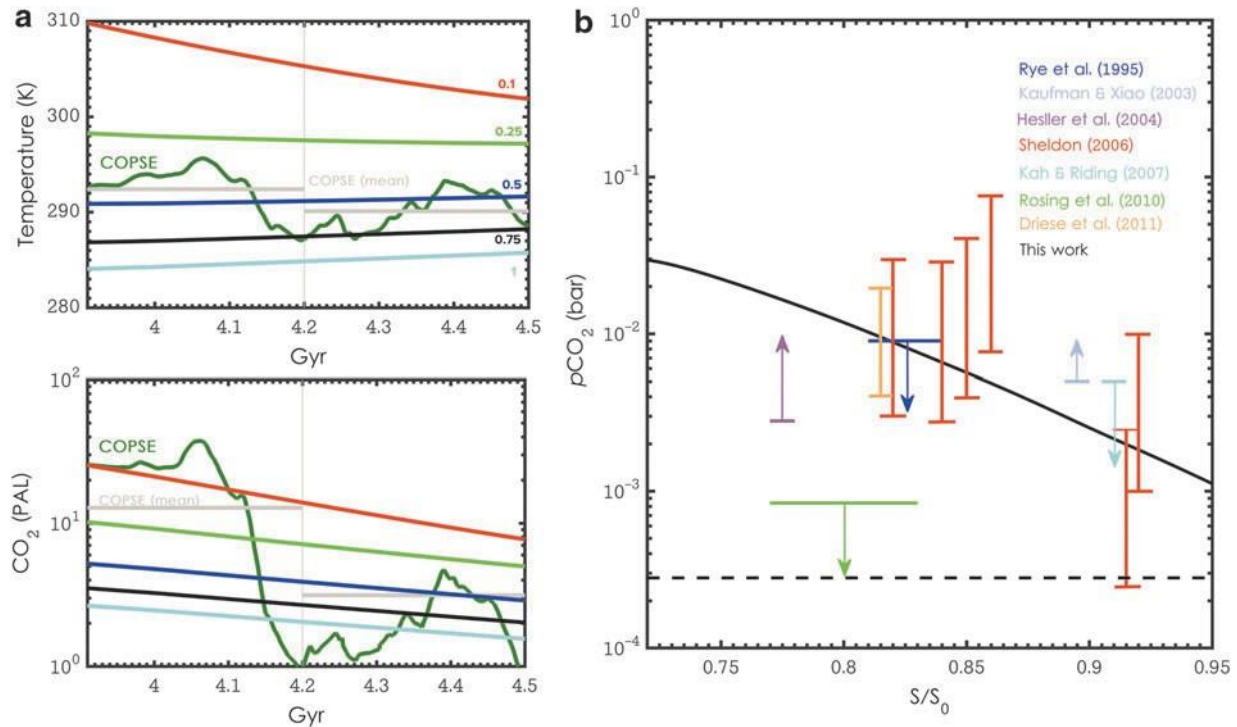
FIG. 2. Ensemble of sensitivity analyses. (a) Model output under differing values of j (biotic enhancement factor, where 1 = present-day weathering rates) compared to results from COPSE model (in dark green, with time-averaged values represented in gray). (b) Modeled p\text{CO}_2 from this work (in bar) (dark line) as a function of time/solar constant, and comparison with empirical estimates of atmospheric carbon dioxide. Figure modified from Feulner (2012). The dashed line indicates preindustrial p\text{CO}_2 (0.000280 bar).
