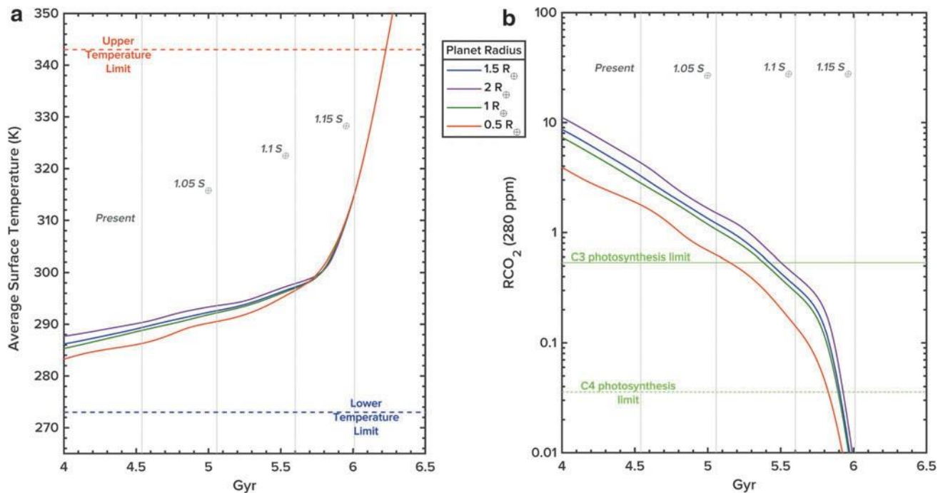
FIG. 3. (a) Average surface temperature as a function of planet size and time, at 1 AU from a brightening Sun. Also displayed are insolation limits as a function of time. (b) Atmospheric p\text{CO}_2 , in preindustrial units ( R\text{CO}_2 = 280 ppm), as a function of planet size and time, at 1 AU from a brightening Sun. Also displayed are insolation limits as a function of time.
