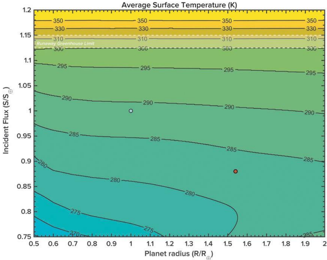
FIG. 4. Contours of average surface temperature in K as a function of planet radius (in Earth-relative units) and incident flux (relative to present-day Earth). Also displayed are current Earth (blue marker) and GJ 667Cc (red marker).
