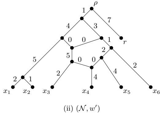
FIGURE 1. Two (weighted) phylogenetic networks on \{r, x_1, x_2, x_3, x_4, x_5, x_6\} .
