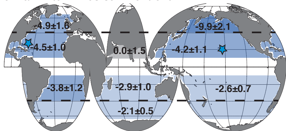
(c) non-thermal winter-minus-summer trend
