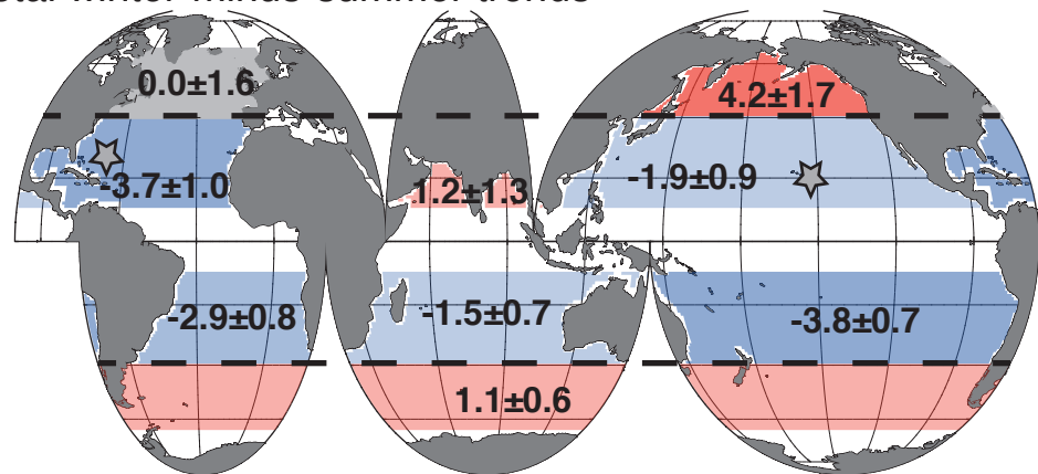
(b) thermal winter-minus-summer trend
