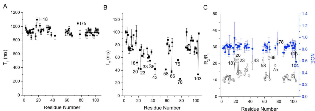
Figure 7: ^{15}\text{N} relaxation parameters for the oxidized Y48H hCc variant acquired at 800 MHz and 288 K. A) T_1 and B) T_2 times plotted against residue number. C) R_2/R_1 ratio (black open circles) and [^1\text{H}]-^{15}\text{N} NOE (blue circles) plotted against residue number.
