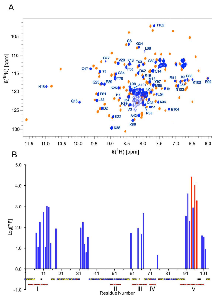
Figure 6: Backbone amide assignments and amide proton H/D exchange analysis of the oxidized Y48H hCc variant. A) An overlay of the 800 MHz [^1\text{H}, ^{15}\text{N}] -HSQC spectrum of the Y48H variant (blue) with the WT protein spectrum (orange) at 288 K. Assignments for most of the assigned backbone amide resonances in the Y48H spectrum are indicated in blue. B) PFs for the Y48H variant plotted against residue number. For the PFs that could be calculated 3 residues underwent fast-exchange ( \log\text{PF} \leq 1 ), 13 medium ( 1 < \log\text{PF} \leq 2 ), 10 slow ( 2 < \log\text{PF} ) and 3 extremely slow-exchange (residual proton occupancy > 80\% after \sim 134 h corresponding to exchange rates < 0.003 \text{ h}^{-1} , shown in red). Secondary structure ( \alpha -helix) is indicated by the bottom red squares with the 5 \alpha -helices numbered I-V, while red squares above represent Pro residues. Unassigned and fast-exchanging residues are indicated in dark blue and yellow squares, respectively. Residues for which PFs could not be calculated due to the slowness of the exchange are indicated with black squares (3 residues).
