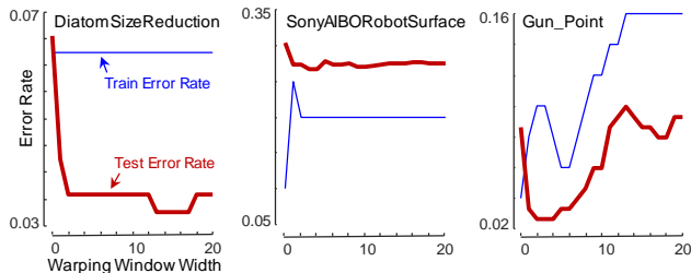
Figure 2. blue/fine : The LOO error-rate of three datasets for increasing values of w . red/bold : The holdout error-rate. In these examples, the holdout accuracies do not track the predicted accuracies.
