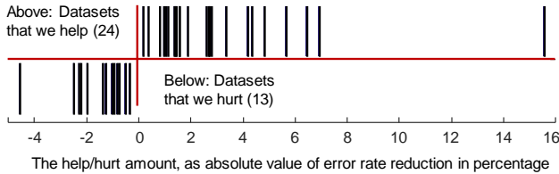
Figure 10. The number of datasets that we help are nearly twice the number of datasets that we hurt .
