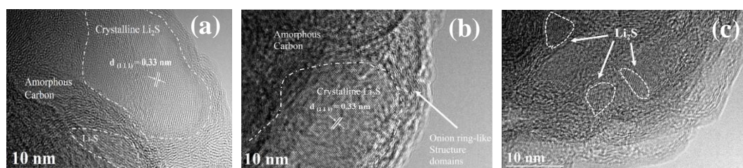
Fig. 3 HRTEM images of the \text{Li}_2\text{S}/26\text{wt}\% \text{C} (a) and \text{Li}_2\text{S}/41 \text{ wt}\% \text{C} (b,c) hybrids.
