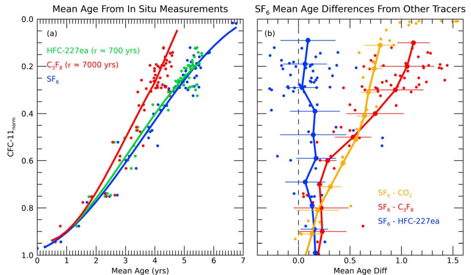
Figure 9. (a) Mean ages calculated from SF 6 , C 3 F 8 , and HFC-227ea in situ measurements from high northern latitude aircraft flights in January–March 2010. The mean ages are plotted as a function of CFC-11 normalized to the tropical average mixing ratio at the surface at the time of the measurements. (b) Differences between mean age calculated from SF 6 and that calculated from C 3 F 8 , HFC-227ea, and CO 2 as a function of normalized CFC-11. The C 3 F 8 and HFC-227ea mean age differences are from the aircraft data shown in Figure 9a, while the CO 2 mean age differences are from the 5 March 2000 balloon flight shown in Figure 2. The error bars are the standard deviations of the mean age differences within each CFC-11 bin.
