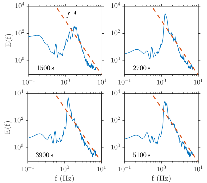
FIG. 2. Temporal evolution of the wave spectrum as a function of the intrinsic frequency. To guide the eye, a power law f^{-4} , corresponding to the prediction of the wave turbulence theory, is also shown as a dashed line.
