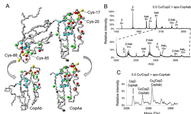
Fig. 3. The interaction of CopAab with CopZ. A) 15 N Chemical shift changes observed upon interaction of 15 N apo-CopAab with unlabelled Cu(I)-CopZ at 1:2 ratio mapped on the apo-CopAab solution structure. NHs cross-peaks broadened beyond detection are shown in red, while those showing measurable changes are shown in green (large NHs chemical shift variations ( \Delta_{\text{avg}}(\text{HN}) > 0.05 \text{ ppm} ) or in cyan (small NHs chemical shift variations ( 0.02 < \Delta_{\text{avg}}(\text{HN}) < 0.05 \text{ ppm} )), where \Delta_{\text{avg}}(\text{HN}) = \{([\Delta\text{H}]^2 + [\Delta\text{N}/5]^2)/2\}^{1/2} . Cys residues of both metal binding sites are also shown in yellow. A rotated view of both CopAa and CopAb domains is shown at the bottom to allow for viewing of the interaction surfaces, which are facing the reader. B) ESI-MS mass spectrum following mixing of 0.5 Cu/CopZ with apo-CopAab. An expanded view of the m/z = 2000 - 2750 region is shown. Each protein envelope is labelled with the corresponding charge state of each peak, as follows: Aab, CopAab monomer; Aab 2 , CopAab dimer; Z, CopZ monomer; Z 2 , CopZ dimer; Z:Aab, CopZ-CopAab complex. C) Deconvoluted mass spectrum of the CopZ-CopAab complex region for the m/z data shown in B). Proteins were in 20 mM ammonium acetate, pH 7.4.
