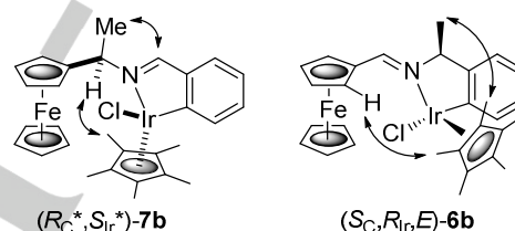
Figure 2. Significant NOE interactions observed for ( R C * , S Ir * )- 7b and ( S C , R Ir , E )- 6b .
