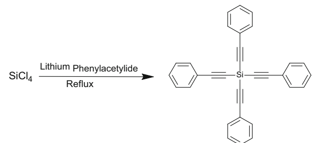
Scheme 1. Synthesis procedure of tetrakis(2-phenylethynyl)silane
