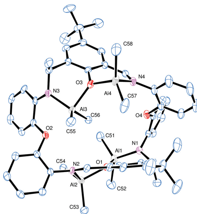
Fig. 7 Molecular structure of [(AlMe_2)_4L^1] \cdot 1\frac{1}{4}toluene \cdot 1\frac{1}{4}hexane (11- 1\frac{1}{4}toluene \cdot 1\frac{1}{4}hexane ), showing the atom numbering scheme. Hydrogen atoms and solvent molecules of crystallisation have been omitted for clarity. This is one of four unique complex molecules in the asymmetric unit. Selected bond lengths (Å) and angles (°): Al1–N1 1.820(3), Al1–O1 1.950(2), Al2–O1 1.857(2), Al2–N2 1.952(2), Al3...O2 2.430(2), Al3–O3 1.997(2), N1–C1 1.469(4), N2–C13 1.286(4), N2–C15 1.276(2), N2–C14 1.442(4), N3–C25 1.381(4), N3–C26 1.473(4), N4–C38 1.288(4), N4–C39, Al1...Al2 3.1695(12), Al1...Al3 5.8984(13), Al1...Al4 7.3100(13), Al2...Al3 5.0994(13), Al2...Al4 7.5339(13), Al3...Al4 3.4600(13); Al1–O1–Al2 112.73(10), Al3–O3–Al4 129.79(12), N1–Al1–O1 95.53(10), O1–Al2–N2 94.72(10).
