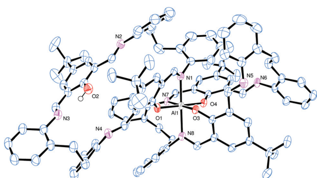
Fig. 6 The molecular structure of [Al(L^5)(L^5H)] \cdot 5MeCN (10-5MeCN), with atoms drawn as 50% probability ellipsoids. Hydrogen atoms, except that on O2 which H-bonds to N3, and MeCN solvent molecules of crystallisation have been omitted for clarity.
