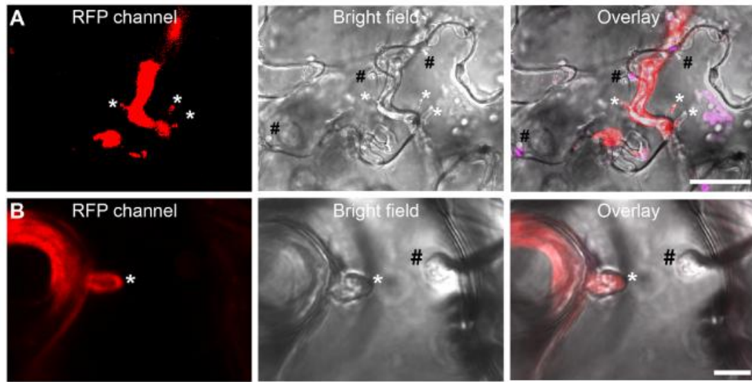
Figure 5. Phytophthora infestans and Albugo laibachii can form haustoria in the same Arabidopsis cell. (A) A. thaliana Col-0 precolonized with A. laibachii was infected with red fluorescent P. infestans 88069td. Inspection by microscopy at 2 dpi revealed the presence of haustoria. (B) Frequently, plant cells were observed to harbor digit-like, red fluorescent P. infestans 88069td haustoria as well as knob-like A. laibachii haustoria. All experiments were performed twice with similar results.
