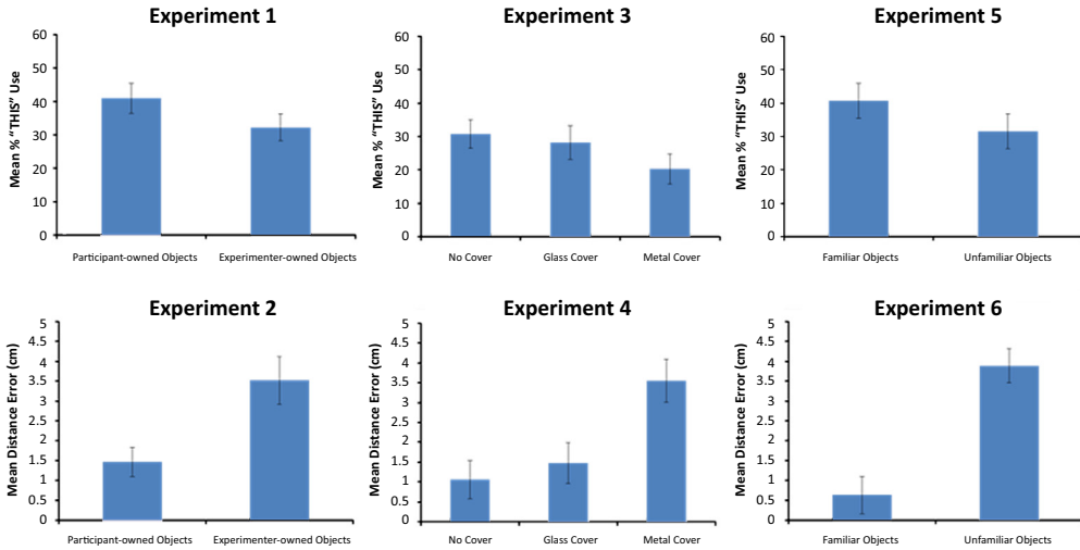
Fig. 3. Main effects of object knowledge found across Experiments 1–6. The top panel shows the results of the demonstrative experiments (mean percentage use of this by condition), and the bottom panel shows the memory results (mean signed distance errors; note that a positive value indicates remembering an object as being further away than it actually was). Error bars represent standard errors of the mean.
