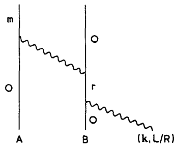
Figure 14. Typical graph for two-group circular dichroism with coupling between the two groups.
