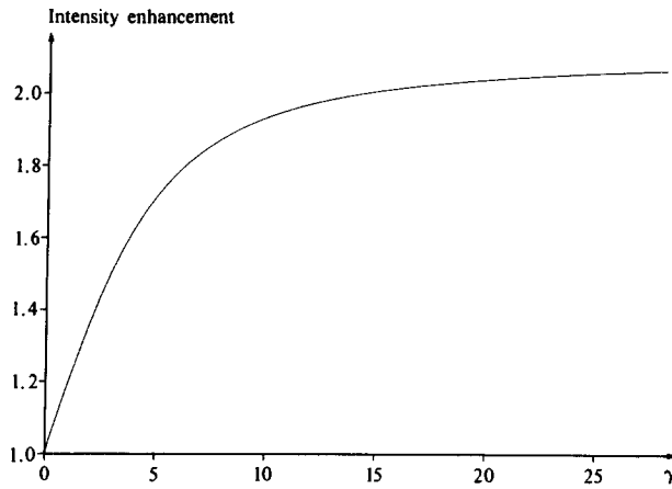
FIG. 5. Enhancement of intensity for a pure weight-0 transition as a function of \gamma = \mu^{00} E_{\text{mol}} / kT .
